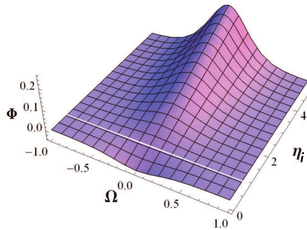
Figure 6. ITG driven mode solitary wave potential against the phase of the soliton \eta and \eta_i .
