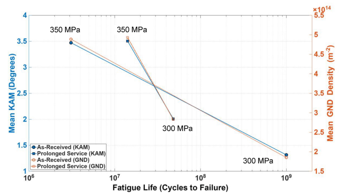
Fig. 9. Quantitative correlation between microstructural strain localisation (measured via mean KAM and GND density) and the statistically averaged fatigue life for the as-received and prolonged-service 10H2M steel across the evaluated stress amplitudes.
