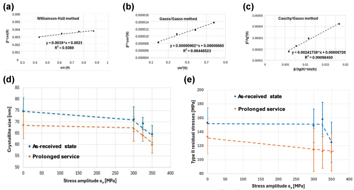
Fig. 14. Methodology for determining the crystallite size (D) and Type II residual (micro-) stress using the Williamson–Hall (a), Gauss/Gauss (b), and Cauchy/Gauss (c) line-profile analysis methods, demonstrated for a non-deformed specimen after prolonged service. The corresponding average values of the ferritic matrix crystallite size (d) and Type II residual stress (e).
