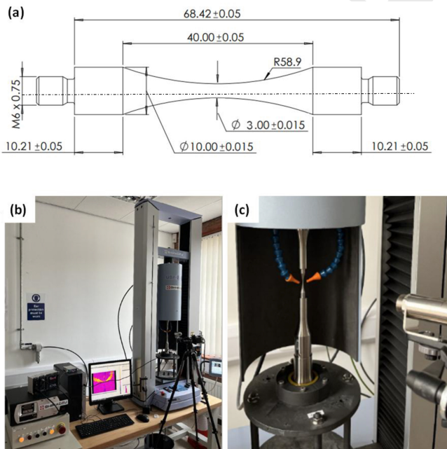
Fig. 2. Engineering drawing of the double-threaded hourglass specimen (a); general view of the experimental setup (b) and close-up view of the specimen (c).
