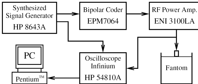
Fig. 3. Diagram of experimental setup.
