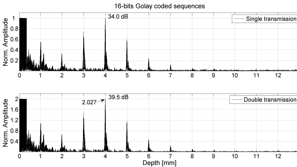
Fig. 5. The centre RF-lines of the tissue phantom obtained by single transmission (top) and double transmission (bottom) of 16-bits Golay sequences.
