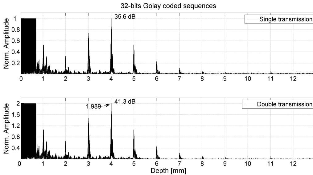
Fig. 6. The centre RF-lines of the tissue phantom obtained by single transmission (top) and double transmission (bottom) of 32-bits Golay sequences.
