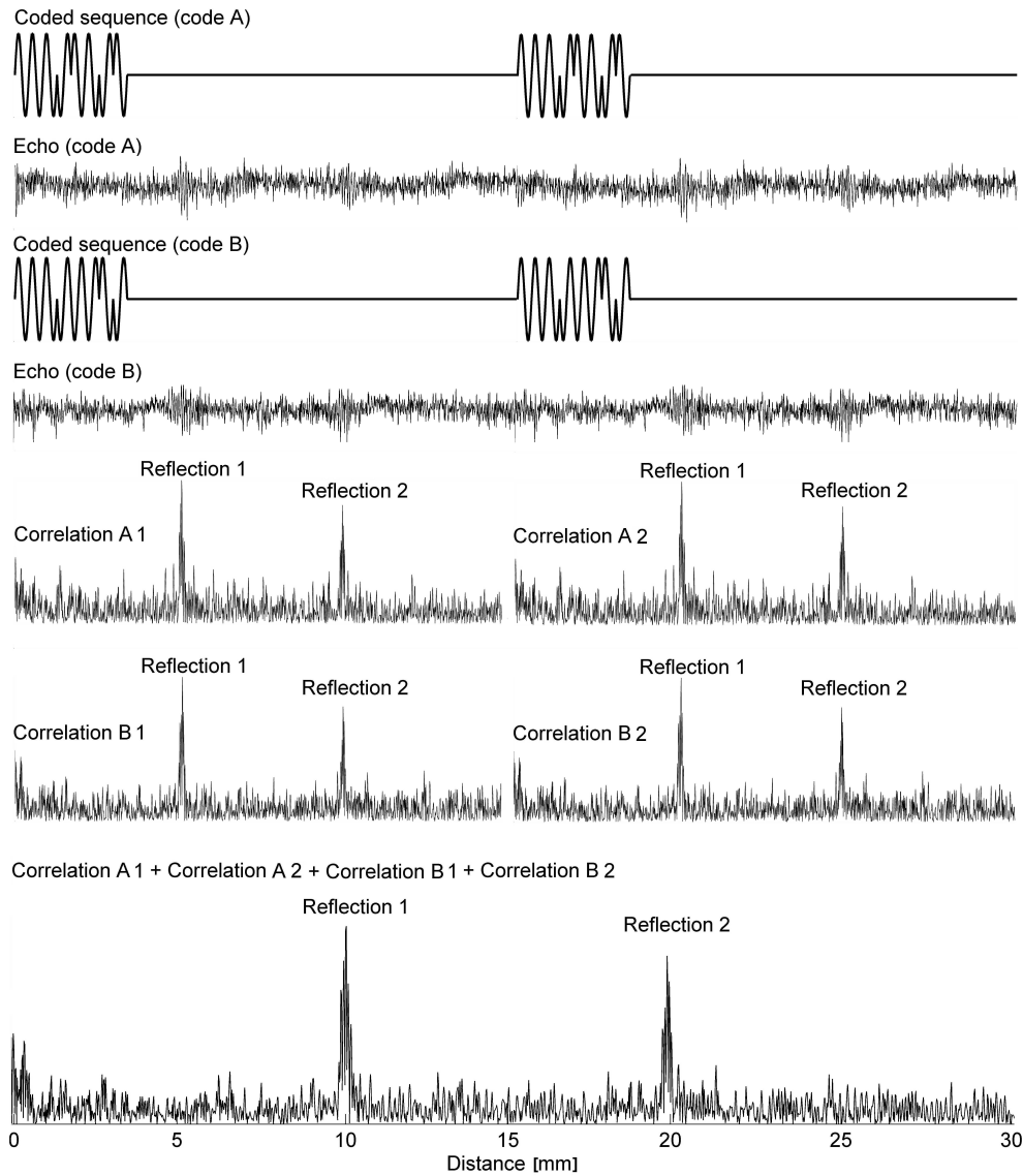
Fig. 1. Double pulse transmission method using Golay complementary sequences.
