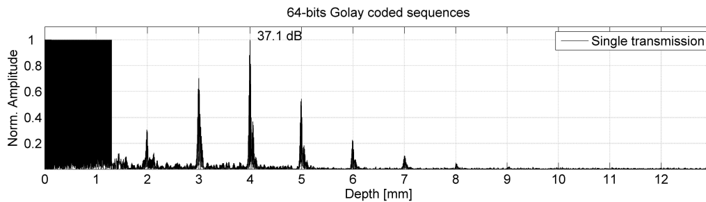
Fig. 7. The centre RF-lines of the tissue phantom obtained by single transmission of 64-bits Golay sequences.
