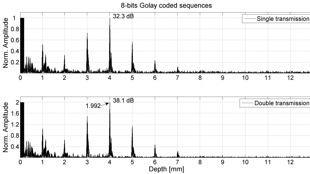
Fig. 4. The centre RF-lines of the tissue phantom obtained by single transmission (top) and double transmission (bottom) of 8-bits Golay sequences.
