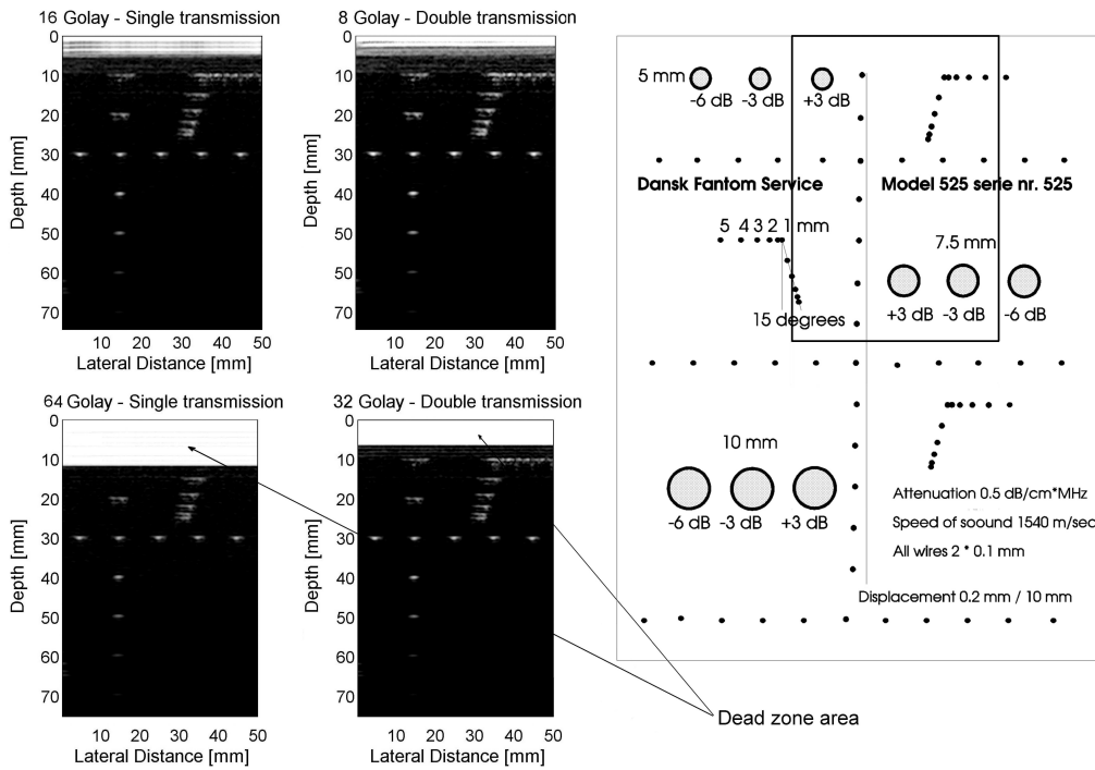
Fig. 8. Comparison of 2D ultrasonic images of the tissue phantom obtained using 8-bits, 16-bits, 32-bits and 64-bits length Golay coded used single transmission and double transmission. Schematic diagram of the examined tissue phantom model 525 . The rectangle marks the scanned area.
