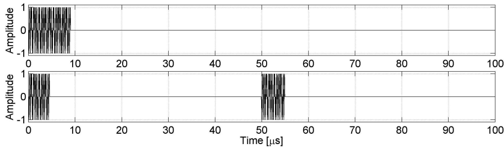
Fig. 2. Transmission of the 32-bits Golay sequence with time duration 8.64 \mu s (top) and double transmission of the 16-bits Golay sequence with time duration 4.32 \mu s (bottom).
