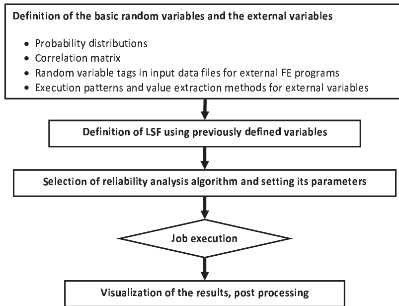
Fig. 1. Major steps of reliability analysis task using STAND
