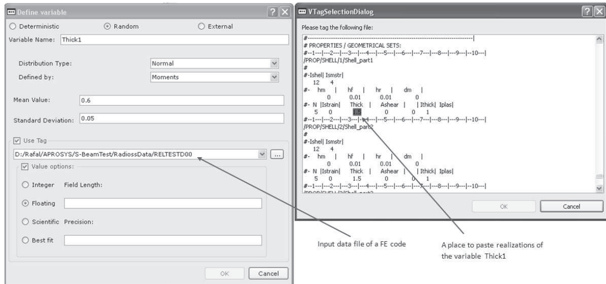
Fig. 3. Associating the random variables with particular locations in the input data files of FE programs
