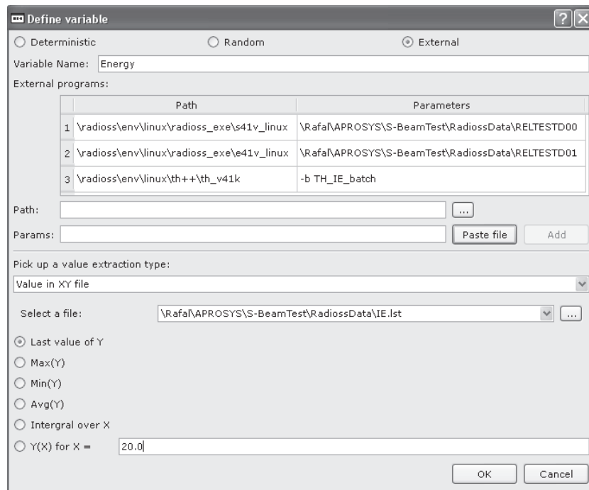
Fig. 4. Interface for external variables definition. A sequence of three programs needs to be executed in order to get the output file as a time history function. The value of the variable is obtained as the last one from the tabulated relationship
