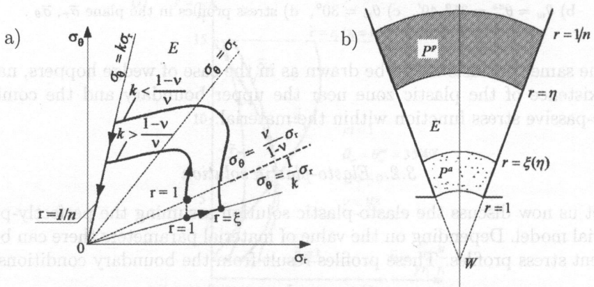
FIG. 6. Stress profiles for the elasto-plastic model: a) stress profiles in the plane \sigma_r, \sigma_\theta , b) plastic and elastic zones within the hopper.
