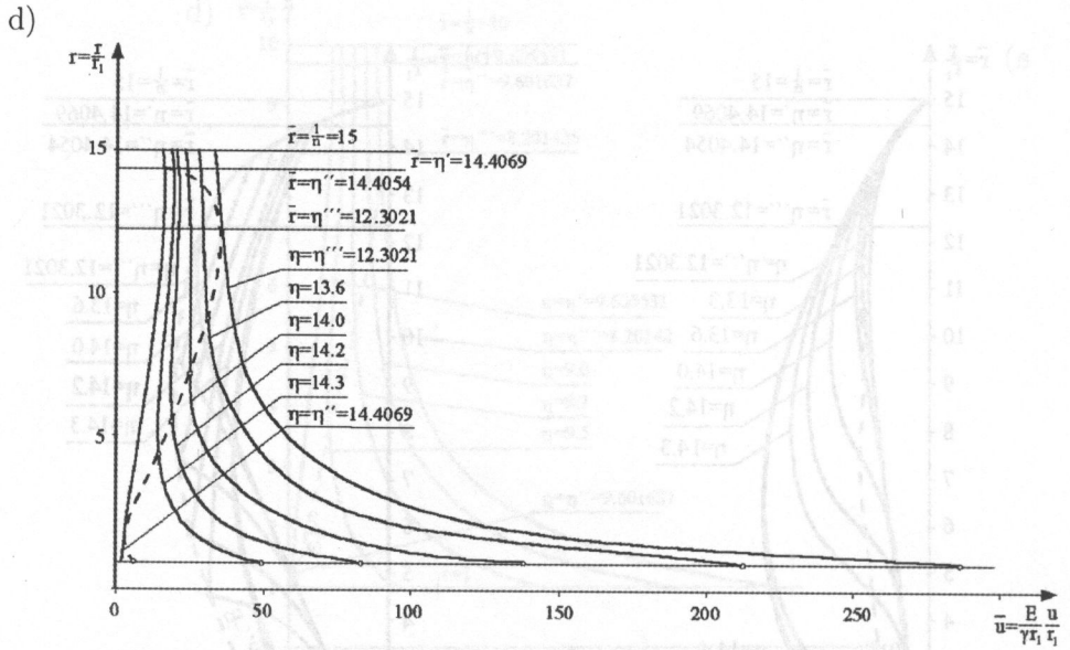
FIG. 10. Stress and displacement evolution during emptying process: a) radial stresses \sigma_r , b) hoop stress \sigma_\theta , c) stress profiles, d) displacement fields; ( \theta_w = 15^\circ , n = 1/15 ).
