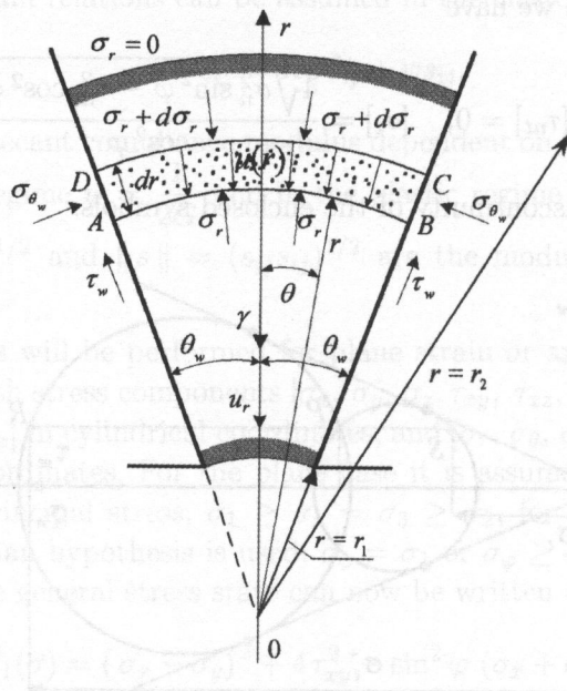
FIG. 3. Simplified radial flow in the hopper: stresses acting on the element ABCD.
