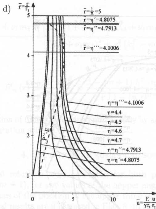
Fig. 8 Stress and displacement evolution during emptying process: a) radial stresses \sigma_r , b) hoop stress \sigma_\theta , c) stress profiles, d) displacement fields; ( m = 0, \mu = 30^\circ, \nu = 1/3, \theta_w = 15^\circ, \nu = 1/3 . As \eta increases the plastic zone propagates and the wall pressure reaches its maximum at the instant when \bar{\sigma}_r = \bar{\sigma}_\theta between I'' and E . There
