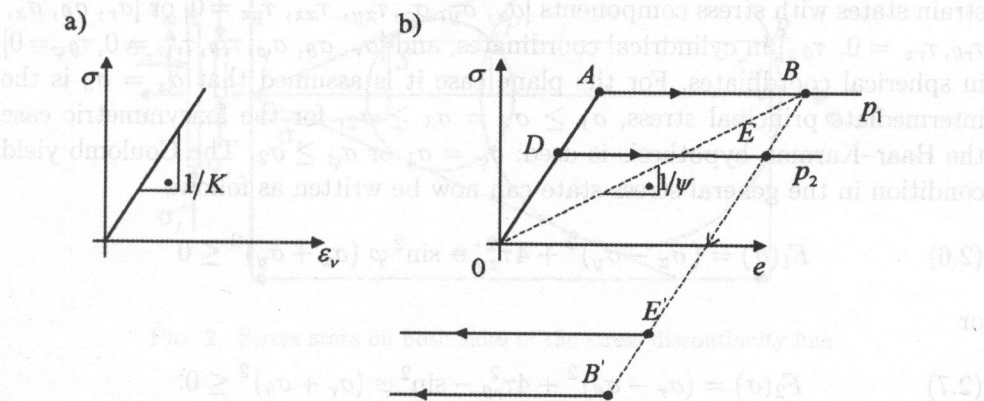
FIG. 1. Linear elastic a) and elastoplastic b) material model.
