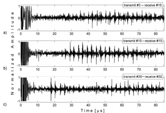
Fig. 5 The recorded by PC RF echo signals: a) element #3 is transmitting – element #15 is receiving, b) #15 transmitting – #15 receiving, c) #30 transmitting – #32 receiving
