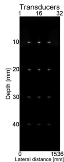
Fig. 3 2D ultrasound phantom image with point targets
