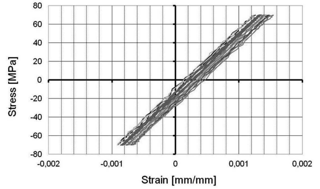
Fig. 4. Hysteresis loops for the cycles over 100 of fatigue tests. Material Al (second series) tested at stress amplitude equal to 70 MPa
