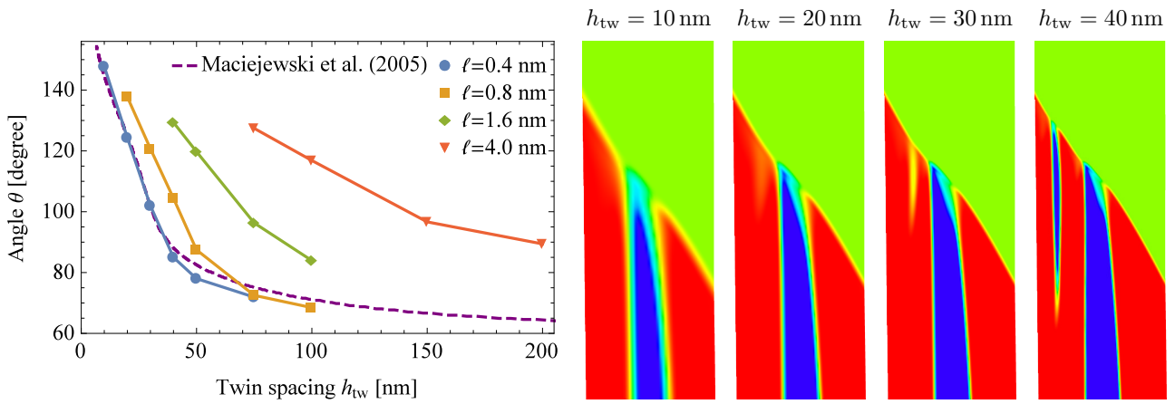
Figure 2. Microstructure M2: dependence of the angle \theta on h_{tw} and \ell . Dashed line depicts prediction of the sharp-interface model [1].
