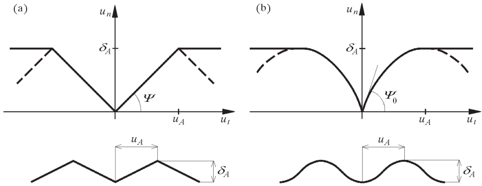
Fig. 15. Dilation curves resulting from the assumption of periodic saw-tooth (a) and sine-shaped (b) asperities
