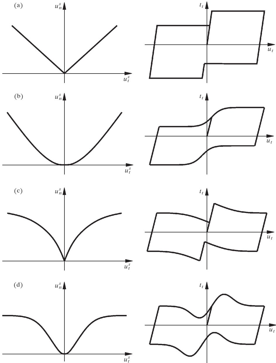
Fig. 17. Configurational dilation: typical dilation curves and resulting cyclic shear response
