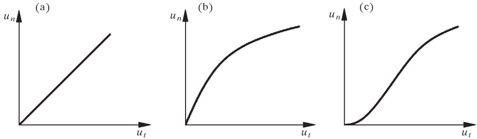
Fig. 5. Typical dilation curves in monotonic direct shear tests
