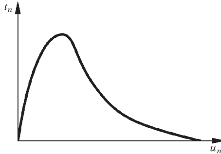
Fig. 2. Typical tensile response of cohesive joints
