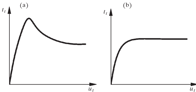
Fig. 4. Typical response to direct shear tests: (a) with and (b) without peak
