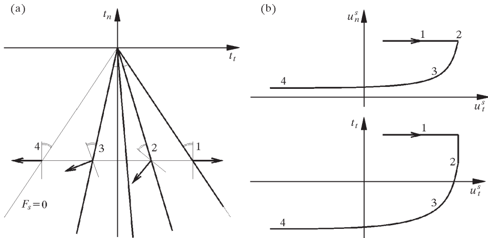
Fig. 23. Rotating cone model (with \Psi_s = 0 ): (a) evolution of the yield surface upon load reversal; (b) dilatancy and frictional response
