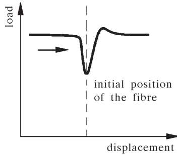
Fig. 8. Reseating drop of the pushing load in a fibre push-back test
