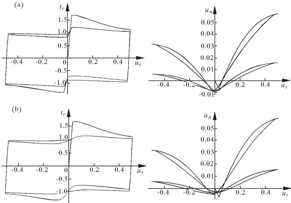
Fig. 20. Configurational dilation with wear effects: friction and dilation response for (a) 1/\bar{\kappa}_g = 0 and (b) 1/\bar{\kappa}_g > 0
