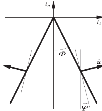
Fig. 10. Limit friction surface of the Coulomb law
