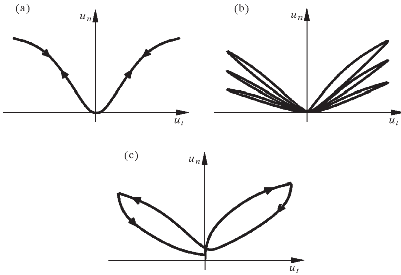
Fig. 6. Cyclic dilatancy response: (a) rock joint under low normal pressure, (b) cyclic degradation of dilatancy, (c) masonry bed joint with a dilatancy drop at load reversal
