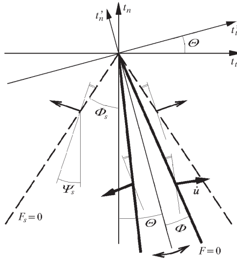
Fig. 22. Rotating yield surface model for granular layer
