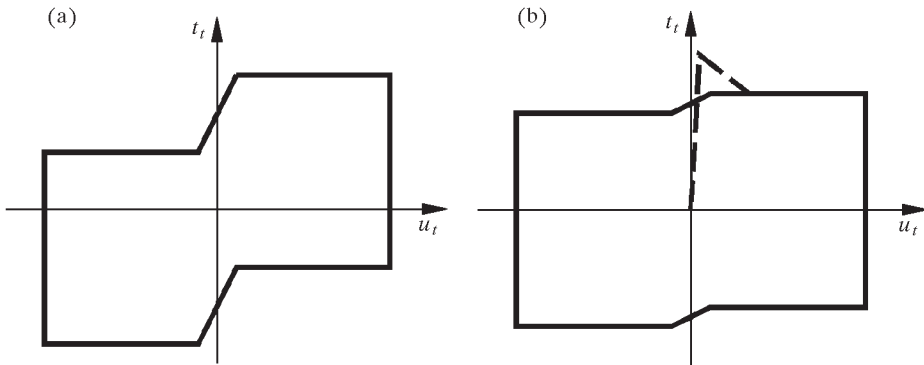
Fig. 7. Idealized friction jump in the vicinity of original mated joint position: (a) strong, (b) weak effect
