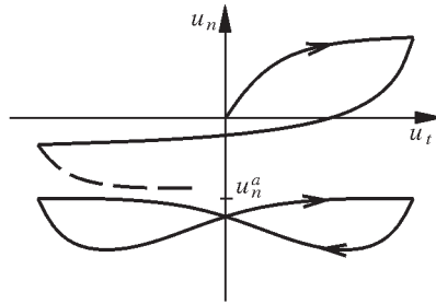
Fig. 24. Rotating cone model for granular layer: dilatancy response to cyclic shearing
