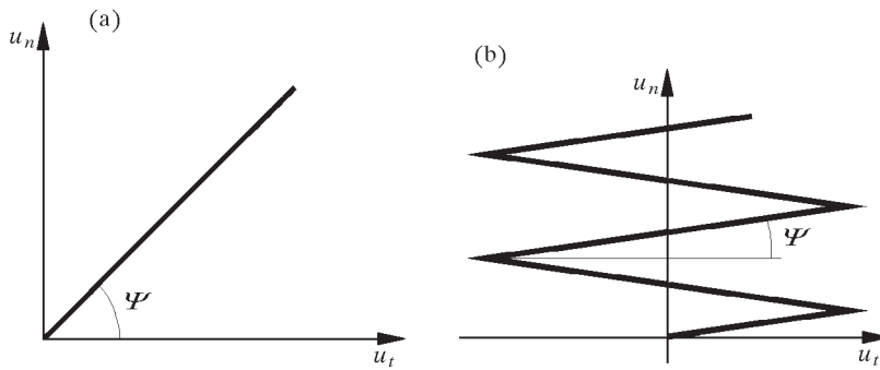
Fig. 11. Dilatancy response of a simple Coulomb law: (a) monotonic and (b) cyclic shearing
