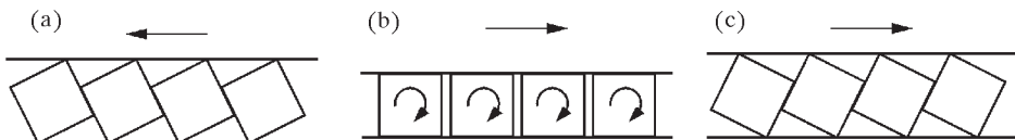
Fig. 21. Configuration rearrangement of particles after the change of sliding direction
