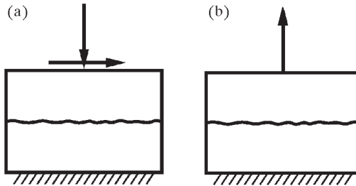
Fig. 1. Scheme of uniform shearing (a) and tensile/compressive (b) tests on joints
