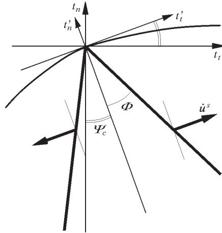
Fig. 16. Friction condition at an inclined contact of primary asperities
