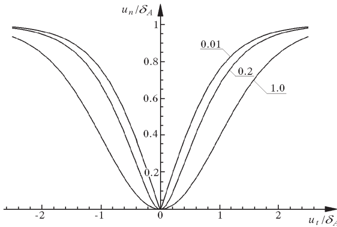
Fig. 18. The effect of g_0 on the dilation curve (3.19) for g_0/\delta_A = 0.01, 0.2, 1
