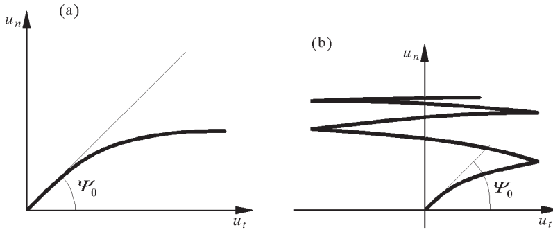
Fig. 12. Dilatancy response of a Coulomb law with decreasing dilation angle: (a) monotonic and (b) cyclic shearing
