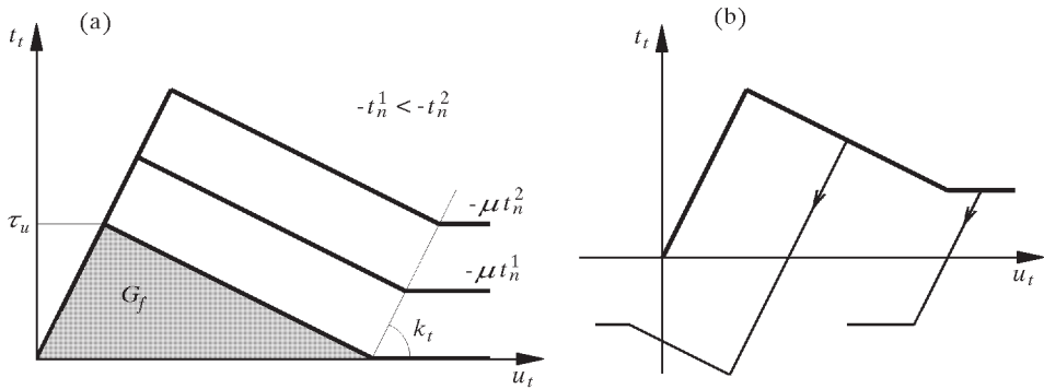
Fig. 13. The response of the cohesive Coulomb law in direct shear: (a) monotonic loading; (b) unloading response
