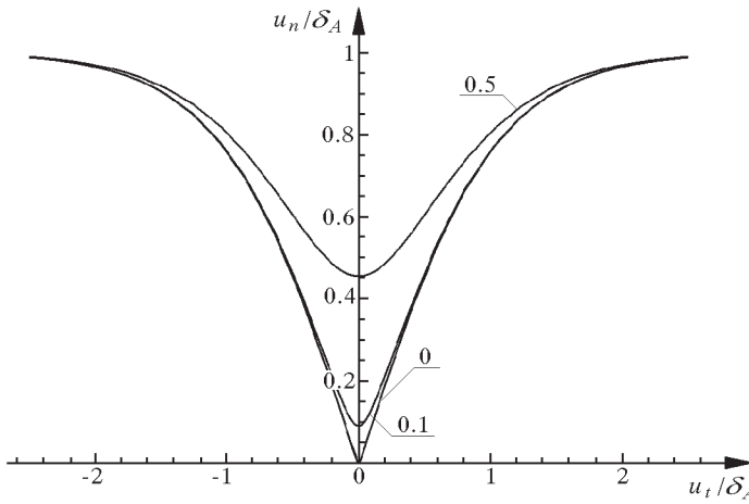
Fig. 19. The effect of g on the dilation curve (3.22) with g_0/\delta_A = 0.01 and for g/\delta_A = 0, 0.1, 0.5
