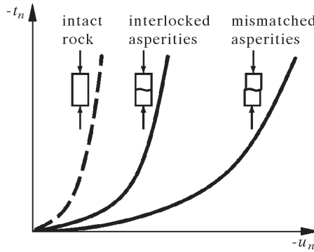
Fig. 3. Typical compressive response of rock joints
