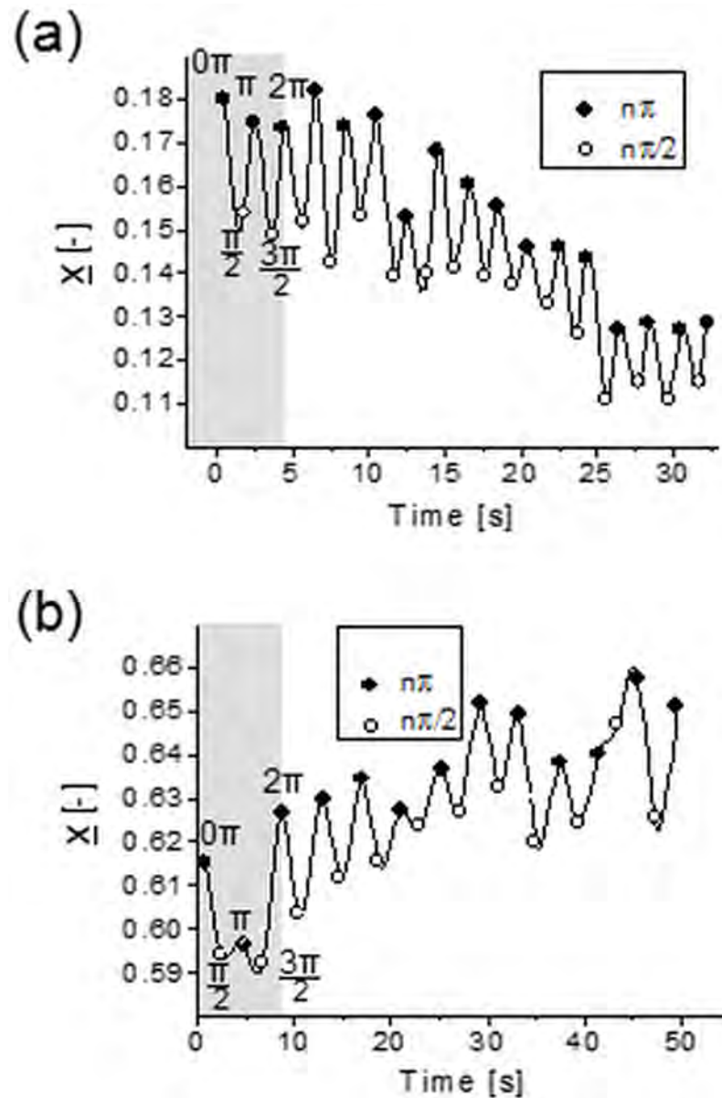
Fig 4. Lateral migration for hydrogel nanofilaments. (a) \Delta toward the channel center ( d = 105 \text{ nm} , L = 41 \mu\text{m} , V_{max} = 250 \mu\text{m/s} , relative migration velocity U_r = 0.85 \cdot 10^{-3} ); (b) \Delta toward the wall ( d = 134 \text{ nm} , L = 54 \mu\text{m} , V_{max} = 132 \mu\text{m/s} , U_r = 0.6 \cdot 10^{-3} ).
