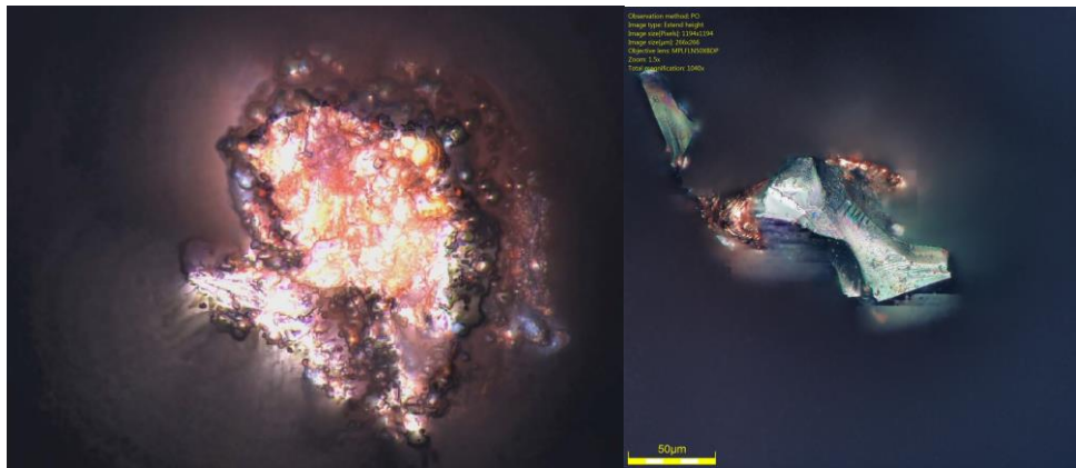
Figure 2. Multifocus optical microscope images of the top of a broken microwire.
