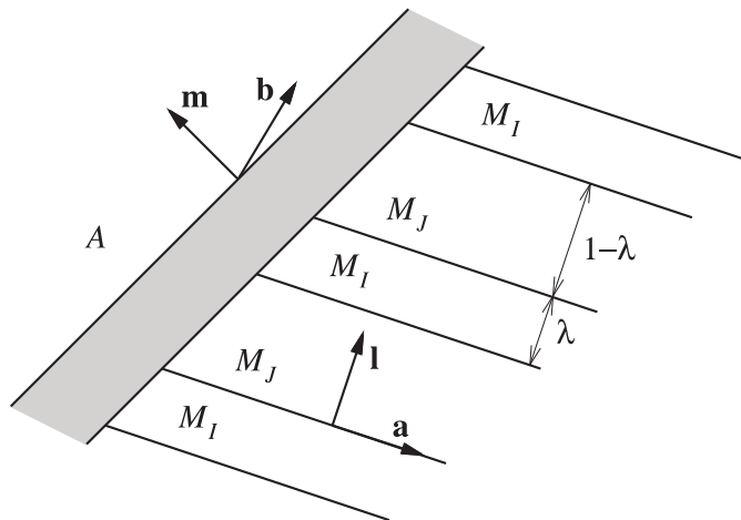
FIG. 1. Microstructure at the austenite–twinned martensite interface ( A – austenite, M_I, M_J – martensite variants, in grey – a transition layer).
