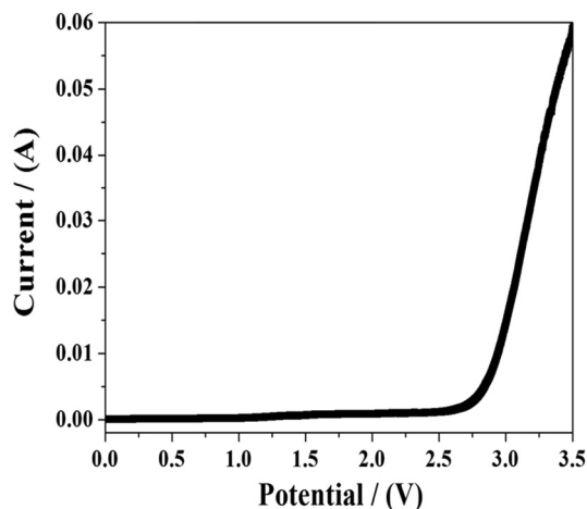
Fig. 9. Linear sweep cyclic voltammetry curves of polymer blend electrolytes with scan rate of 5 \text{ mV s}^{-1} for a cells, (a) SS||PVdF(HFP)-PMMA (80:20) (20 wt%)-[NaSCN] (80 wt%) |SS recorded at room temperature.
