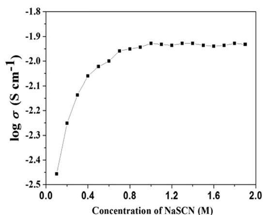
Fig. 5. Variation of electrical conductivity ( \sigma ) of liquid electrolytes (a) NaSCN-DMF as a function of varying salt concentration NaSCN respectively.
