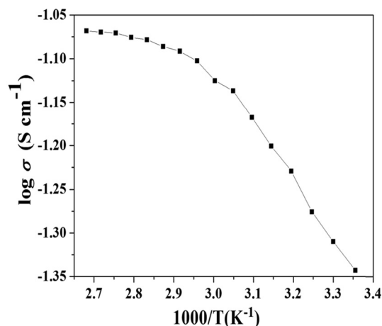
Fig. 8. Temperature dependence ionic conductivity of (a) [PVdF(HFP)-PMMA (80:20)] (20 wt%)-[NaSCN (1 M)] (80 wt%) polymer blend electrolytes.
