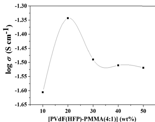
Fig. 7. Variation of ionic conductivity of blend polymer electrolyte (a) PVdF(HFP)-PMMA-NaSCN as a function of different weight percent of [PVdF(HFP)-PMMA] (4:1) polymer blend concentration.
