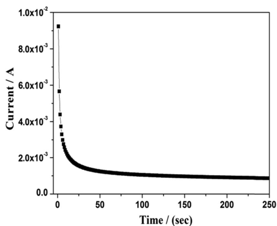
Fig. 10. Polarisation current as a function of time of polymer blend electrolytes of cell SS||PVdF(HFP)-PMMA (80:20) (20 wt%)- [NaSCN] (80 wt%) |SS at room temperature.
