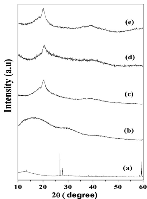
Fig. 1. X-ray diffraction (XRD) spectra of (a) Pure NaSCN, (b) pure PMMA film, (c) pure PVdF(HFP) Film, (d) PVdF(HFP)-PMMA (4:1) film, (e) [PVdF(HFP)-PMMA (4:1)] (20 wt%)-[NaSCN (1 M)] (80 wt%).
