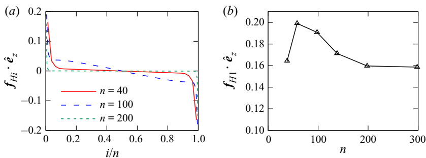
Figure 2. Hydrodynamic forces normal to the fibre, acting on bead i , calculated from (2.15) with the GRPY model of the hydrodynamic interactions. (a) Spatial distribution of the forces on the beads along the fibre. (b) The force on the first bead as a function of the fibre aspect ratio n .
