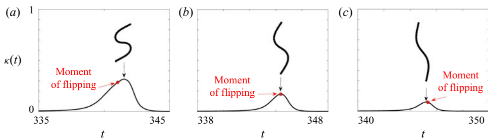
Figure 17. Maximum local curvature \kappa(t) and characteristic fibre shapes at the time \tau_{b2} of the maximum curvature, shown for n = 40 and (a) A = 483.3 , (b) A = 720.6 , (c) A = 880.4 . For the global bending mode, the maximum of the local curvature is observed at the flipping moment or later, as in (b, c).
