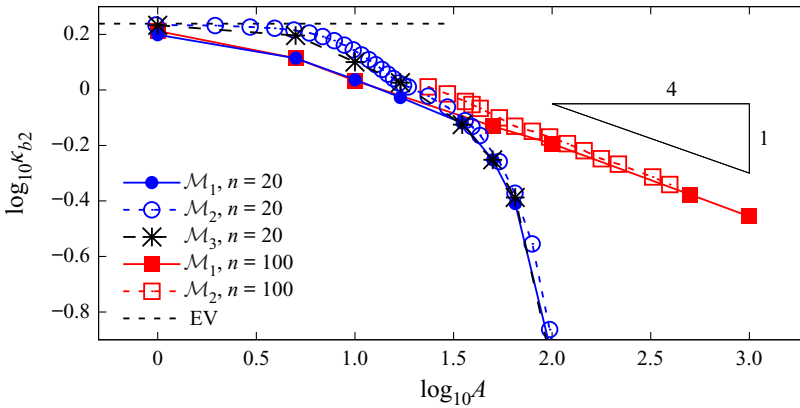
Figure 15. Comparison of three bead models of a flexible fibre. The maximum curvature \kappa_{b2} vs. bending stiffness A , evaluated with the use of the models \mathcal{M}_1 (filled symbols), \mathcal{M}_2 (empty symbols) and \mathcal{M}_3 (stars). The EV limit is marked as the horizontal dashed line.
