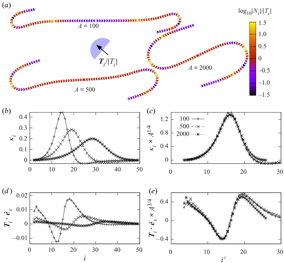
Figure 11. Instantaneous distribution of forces and curvatures on individual beads (fibre statics) for three locally bent fibres with n = 100 and A = 100, 500, 2000 . (a) Shapes of the fibres. The colour coding shows the ratio of the normal |N_i| to the tangential |T_i| force components acting on each bead i , represented as a hemisphere. The orientation of the hemispheres shows the direction of T_i . (b) Curvature \kappa_i on bead i along the fibre. (c) Rescaled curvature as a function of rescaled position i' = (i - i_0)A^{-1/4} along the fibre. (d) Tangential forces T_i \cdot \hat{e}_s acting on beads i – the discrete analogue of the tension’s derivative \sigma_s for the elastica. (e) Rescaled T_i \cdot \hat{e}_s as a function of i' .
