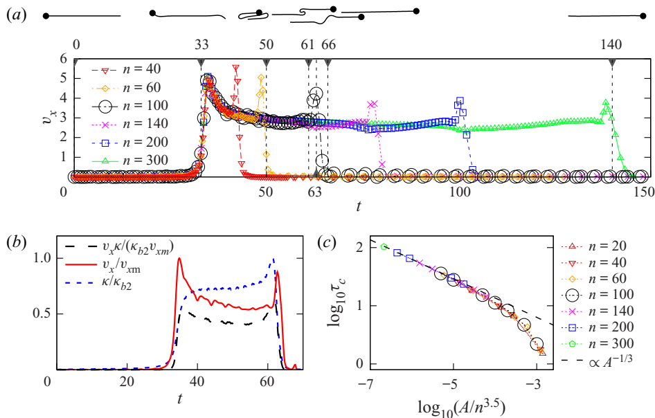
Figure 12. The curling motion. Results from the bead model \mathcal{M}_1 . (a) The x component v_x of the first bead velocity as a function of time for A = 100 and different aspect ratios n . The enlarged black circles represent the fibre of aspect ratio n = 100 (shown in figure 3). The schematics above the plot show the shapes for n = 100 at times marked with vertical dashed lines; the first bead is marked with a dot. (b) Comparison of v_x(t) (normalized with the maximum observed value v_{xm} ) with \kappa(t) (normalized with the maximum curvature \kappa_{b2} ), for A = 100 and n = 100 . (c) Scaling of the curling time \tau_c as a function of A/n^{3.5} , found empirically.
