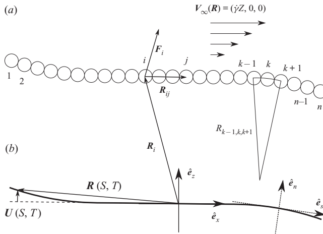
Figure 1. Models of a fibre in shear flow and the notation. (a) The bead model. (b) The elastica model.
