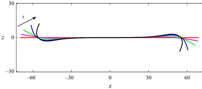
Figure 8. A typical evolution of the shapes of a flexible fibre in an early stage of bending. Here, n = 140 and A = 1000 . The consecutive time instants shown are t = 50, 66, 69, 70, 70.5 , with the last one approximately equal to \tau_b .
