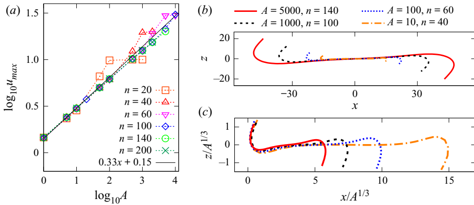
Figure 9. Maximum deflection u_{max} of the fibre tip, defined as z_1(t_{max}) at the time t_{max} of the first maximum, evaluated numerically from the bead model \mathcal{M}_1 . (a) u_{max} as a function of A for different n , with the approximate scaling \propto A^{1/3} . (b) Shapes of fibres at t_{max} for different A and n . (c) Rescaled shapes of fibres from (b), translated to overlay the bending left ends.
