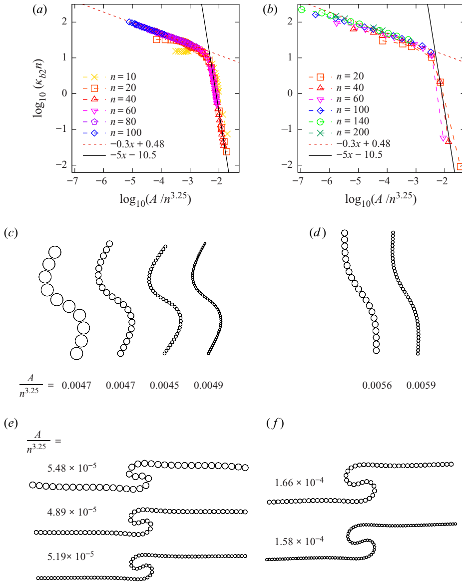
Figure 13. Universal similarity scaling of fibre shapes, evaluated with the model \mathcal{M}_2 , (a,c,e), and with the model \mathcal{M}_1 , (b,d,f). The maximum curvature \kappa_{b2}n , scaled by the inverse of the fibre length, can be approximated as a universal function of A/n^{3.25} , as shown in (a,b) in the log–log scale. The regimes of local and global bending correspond to a more flat and a more steep straight line, respectively. As shown in figure 13(c–f), in both regimes the shapes of fibres are almost the same for approximately the same values of A/n^{3.25} (as indicated). In (c) (n, A) = (10, 8.4), (20, 79.4), (40, 720.6), (60, 2922.5) , in (d) (n, A) = (20, 100), (40, 1000) , in (e) (n, A) = (40, 8.8), (60, 29.4), (80, 79.4) and in (f) (n, A) = (60, 100), (100, 500) .
