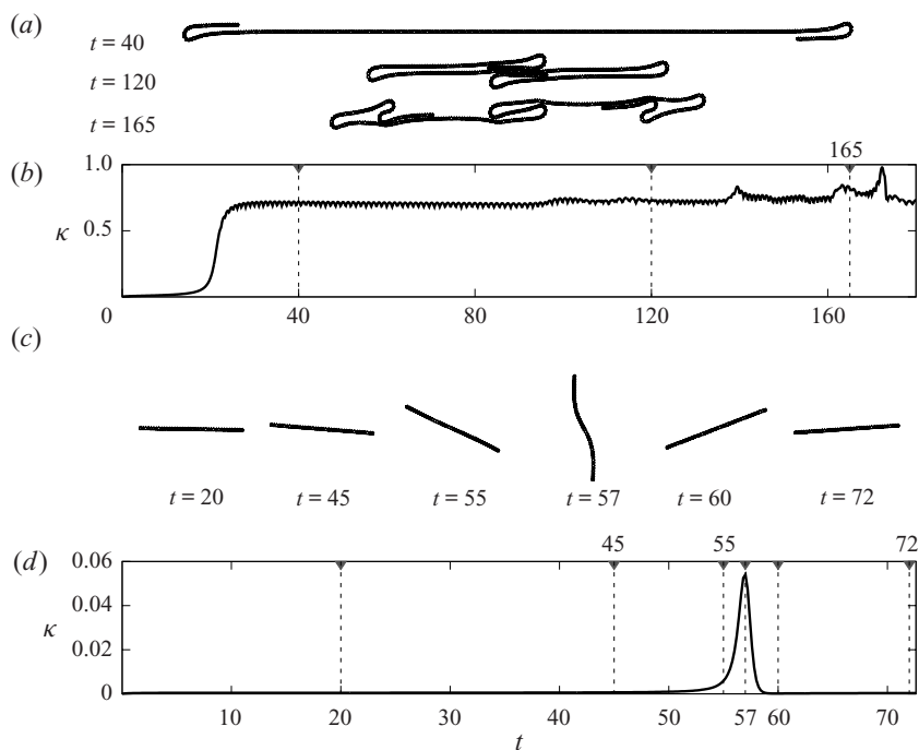
Figure 4. Differences in the evolution of long, very flexible fibres and short, very stiff fibres (based on the model \mathcal{M}_1 ). (a) Shapes of a long, flexible fibre with n = 300 , A = 10 . (b) Curvature of the fibre from (a) versus time. The vertical marks correspond to the shapes from panel (a). (c) Shapes of a short, stiff fibre with n = 40 , A = 1000 . (d) Curvature of fibre from (c). The triangle symbols with vertical dashed lines correspond to the times for which the corresponding shapes are shown in panel (c).
