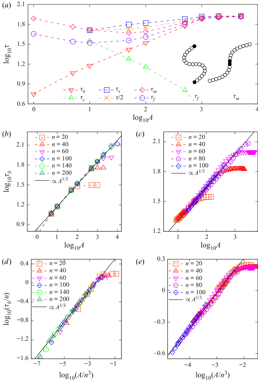
Figure 5. Characteristic time scales in the fibre motion. (a) Comparison of time scales of the fibre motion: the bending time \tau_b , the stretching time \tau_s , the curling time \tau_c , the flipping time \tau_f and the turning time \tau_m for n = 60 and the model \mathcal{M}_1 . Insets show the shapes for the times \tau_f and \tau_m . (b,c) Bending time \tau_b as a function of A for different n from the models \mathcal{M}_1 and \mathcal{M}_2 , respectively. The solid lines show \tau_b \propto A^{1/3} . In (b) the best linear fit is (0.335 \pm 0.002) \log_{10} A + 0.845 \pm 0.005 . (d,e) Bending time \tau_b normalized by n is an almost universal function of A/n^3 , as confirmed by the numerical data from the models \mathcal{M}_1 and \mathcal{M}_2 , respectively.
