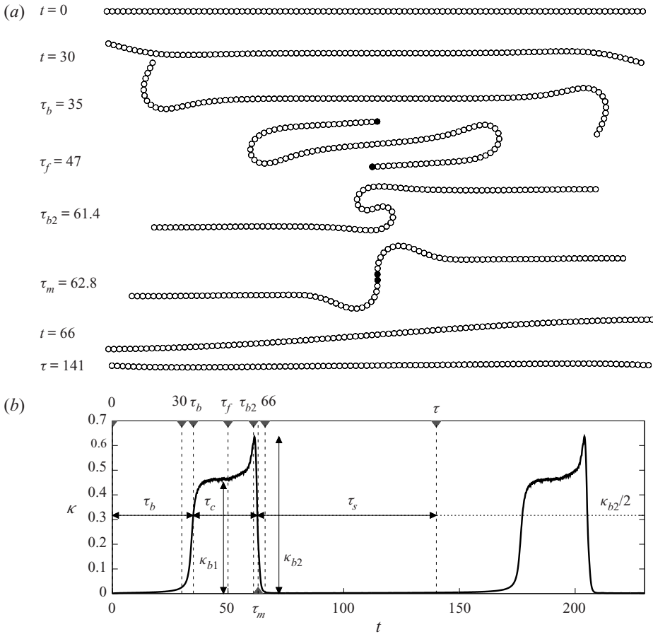
Figure 3. A typical evolution of the shape of a flexible fibre with aspect ratio n = 100 and a moderate bending stiffness A = 100 (based on the model \mathcal{M}_1 ), starting from a straight fibre aligned with the flow. (a) Shapes of the fibre. The circles represent the beads actual scale along the fibre. The black circles highlight the end and middle beads during \tau_f and \tau_m . (b) Maximum local curvature \kappa(t) . Time instances corresponding to the shapes from (a) are marked with dashed vertical lines.
