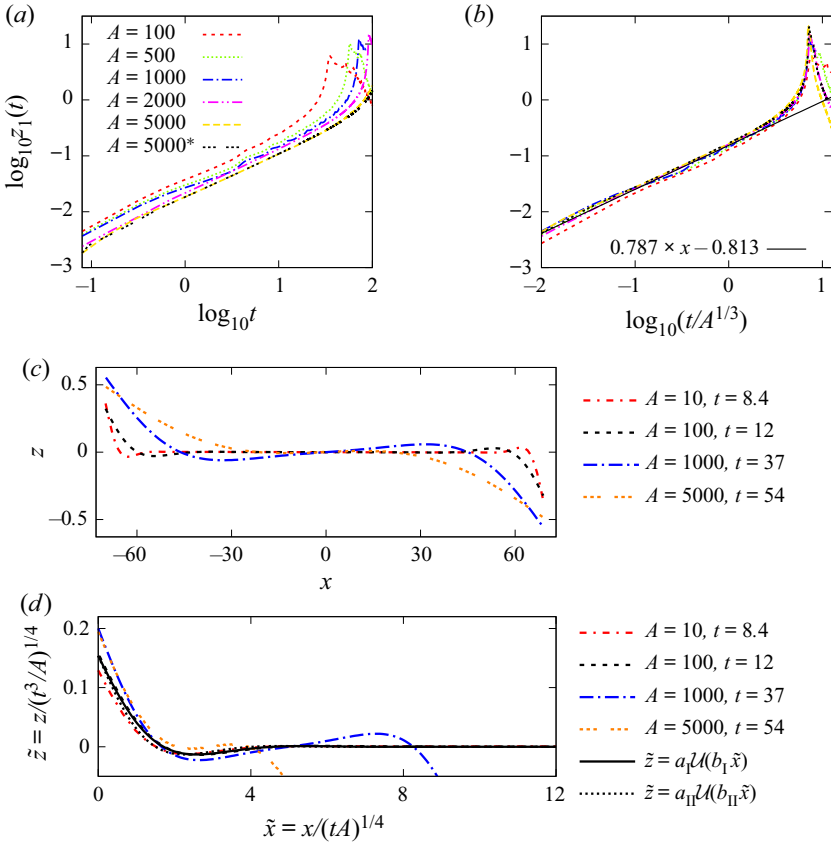
Figure 7. Scalings in the numerical simulations for small deflections. (a) Height z_1(t) of the fibre tip above the horizontal line passing through the centre of the fibre (from the \mathcal{M}_1 model). Fibres have n = 100 , except the fibre denoted with * that has n = 140 . (b) Height z_1(t) from panel (a) as a function of the rescaled time t/A^{1/3} (in log–log scale). The black solid line comes from a fit to all \mathcal{M}_1 data with n \geq 60 , A \geq 50 for times t/A^{1/3} < 0.1 . (c) Shapes of fibres from the bead model \mathcal{M}_1 for n = 140 and different A at arbitrarily chosen times at the end of the regime of the similarity solution. (d) Shape of fibres from panel (c), scaled according to the similarity solution z_1(t) \approx u(s, t) , with u given by (4.6), and translated to approximately overlay the left ends. The numerically obtained shapes are superimposed onto theoretically calculated shapes a_k \mathcal{U}(b_k \tilde{x}) , k = \text{I, II} , with \mathcal{U} given by (4.9) and the coefficients a_k, b_k given in terms of \mathcal{F} and \eta which result from approaches I and II to compare between the bead model and the elastica, given in (4.13)–(4.15) and (4.16), (4.17), respectively.
