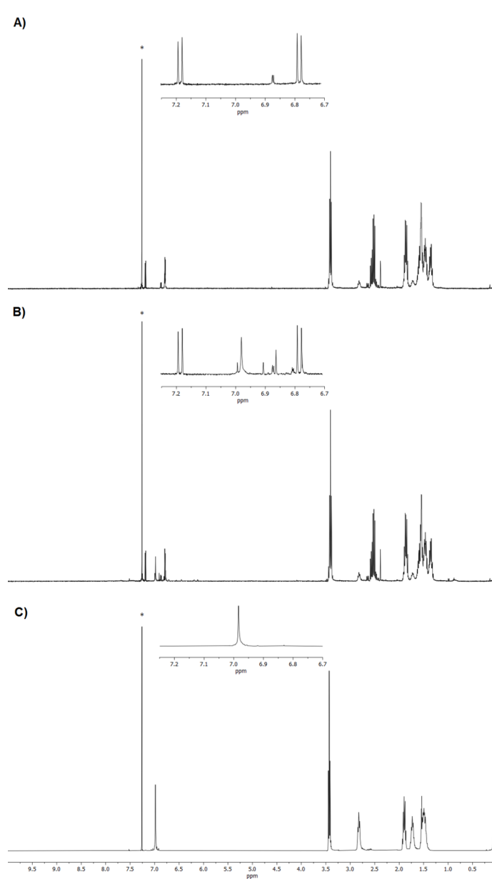
Figure 1. 1 H-NMR spectra of PT6Br after 30 min (A), 60 min (B) and 90 min (C). Asterisk: solvent resonance (CDCl 3 ). Inset: expansion of the aromatic region.
