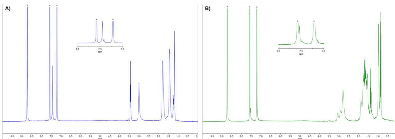
Figure 2. 1 H-NMR spectra of double-cable copolymers, P[(T6Br)-co-(T6F)] (blue line), (A) and P[(T6buP + )-co-(T6F)] (green line), (B). Asterisk: solvent resonance pyridine-d 5 . Inset: expansion of the aromatic region.
