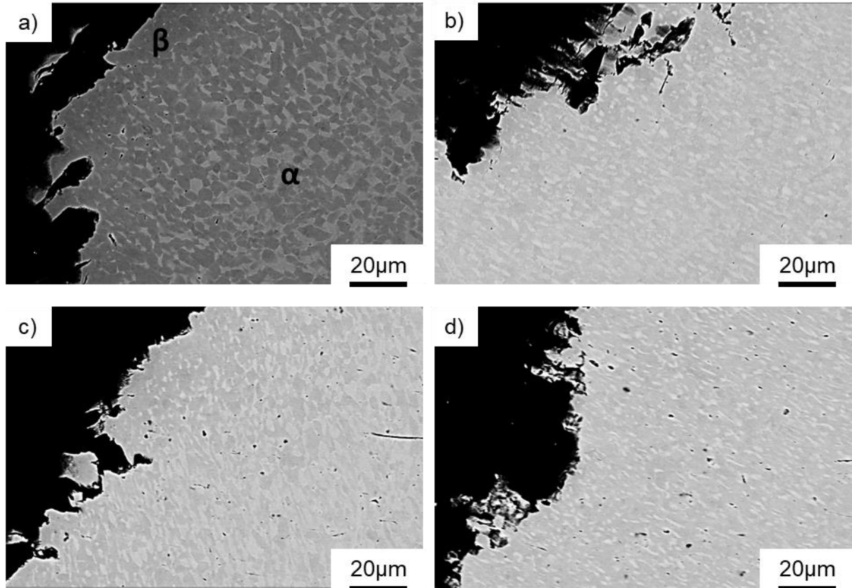
Fig. 2. Fracture area of material subjected to 950°C using slow heating (a) and fast heating (b) conditions; and material subjected to 900°C using slow heating (c) and fast heating (d) conditions.
