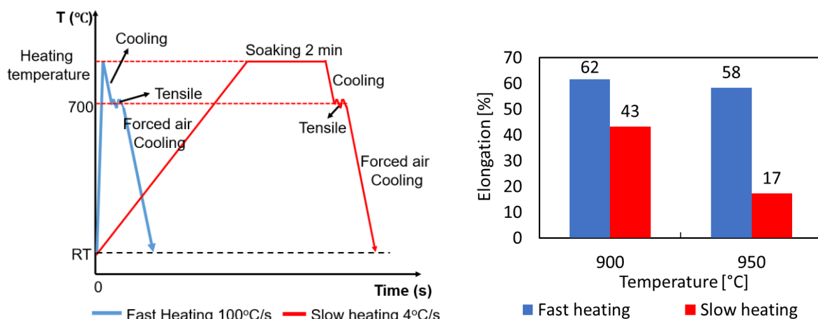
Fig. 1. Non-isothermal tensile tests program (a); effect of heating temperature on elongation (b).
