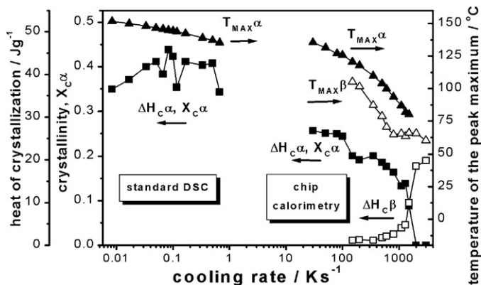
Fig. 2. Heat of crystallization, \Delta H_C , and the temperature of peak maximum, T_{MAX} , of \alpha and \beta peaks as a function of cooling rate. Crystallinity of \alpha phase determined with the enthalpy of melting \Delta H^0_{\alpha} = 104.5 \text{ J/g} [10]. DSC results obtained on samples weighing ca. 7 mg.
