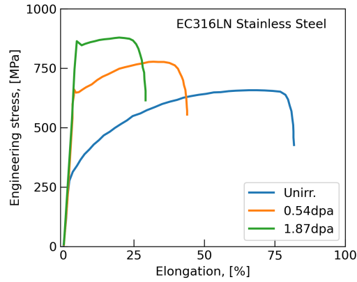
Figure 5: Engineering stress–strain curves of EC316LN stainless steel after irradiation to labeled doses in spallation environments [Byun et al., 2002]
