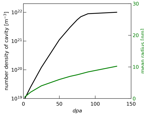
Figure 4: Density of cavity and average cluster size as a function of irradiation dose, based on [Courcelle et al., 2016]
