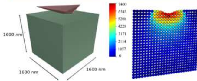
Distribution of equivalent HMH stress at maximum indentation depth for 1.32 dpa
