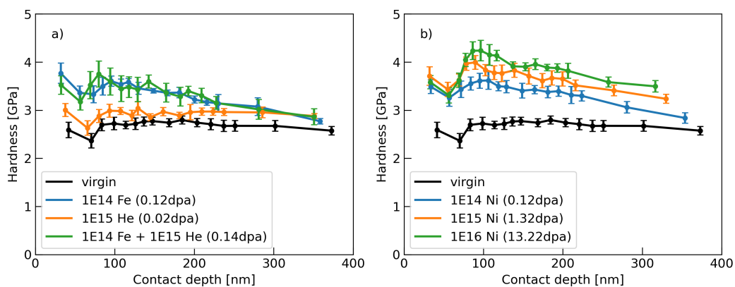
Figure 9: Hardness variation as a function of contact depth for 310SS irradiated with a) Fe and Fe+He ions and b) Ni ions
