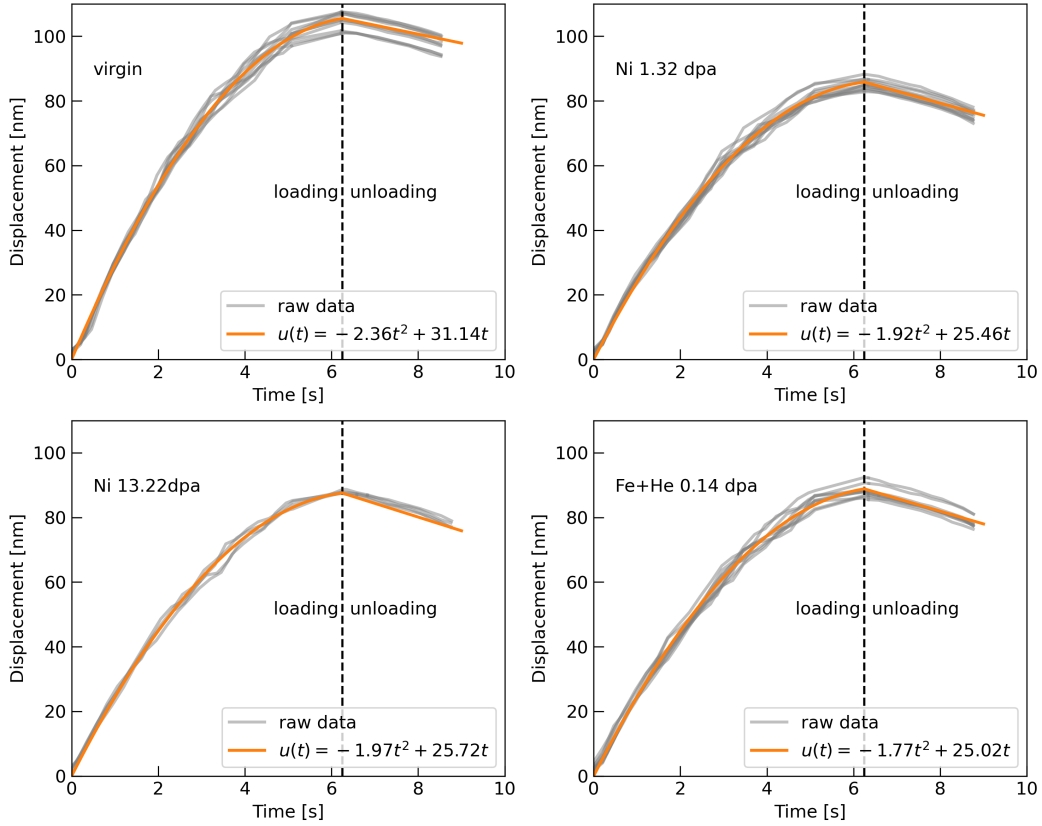
Figure 14: Fitted analytical curves for displacement history of the indenter
