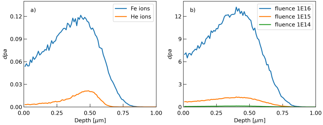
Figure 6: Simulated irradiation damage (in dpa ) as a function of target depth for a) 1.5 MeV Fe ions and 160 keV He ions b) 1.5 MeV Ni ions at the fluence of 1E14, 1E15 and 1E16 ions/cm -2
