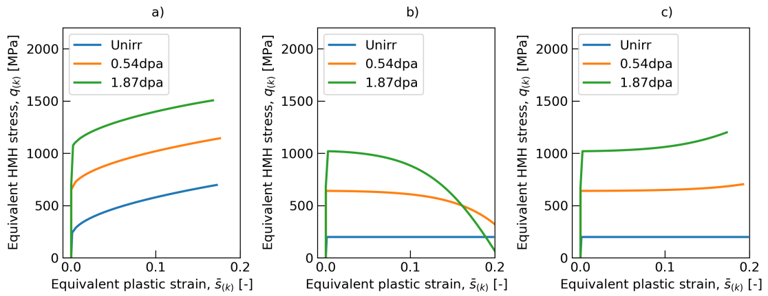
Figure 11: Evolution of the equivalent HMH stress as a function of equivalent plastic strain with selected a) isotropic hardening b) porosity-based softening c) irradiation hardening for different initial level of irradiation
