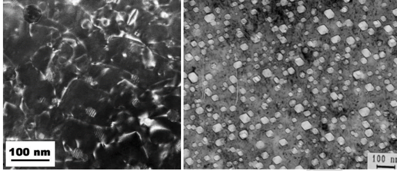
Figure 3: a) TEM image showing dislocation loops, precipitates and voids in irradiated HT9 ferritic/martensitic steel at 155 dpa [Sencer et al., 2009] b) voids observed in irradiated austenitic stainless steel EI-847 at 73 dpa [Porollo et al., 1998]
