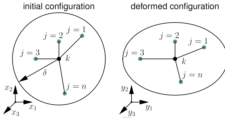
Figure 1: Peridynamics neighbourhood of the material point k . before and after applied deformation
