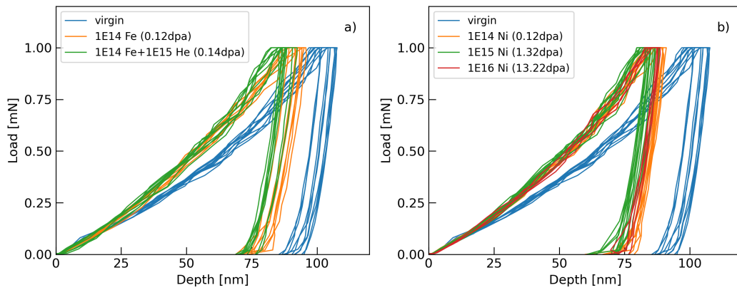
Figure 8: Load – displacement curves on a) virgin; Fe ion-irradiated 310SS specimen up to 0.12 dpa ; and Fe+He ion-irradiated 310SS specimen up to 0.14 dpa ; b) virgin and Ni ion-irradiated 310SS specimen for three value of irradiation dose 0.12 dpa , 1.32 dpa and 13.22 dpa
