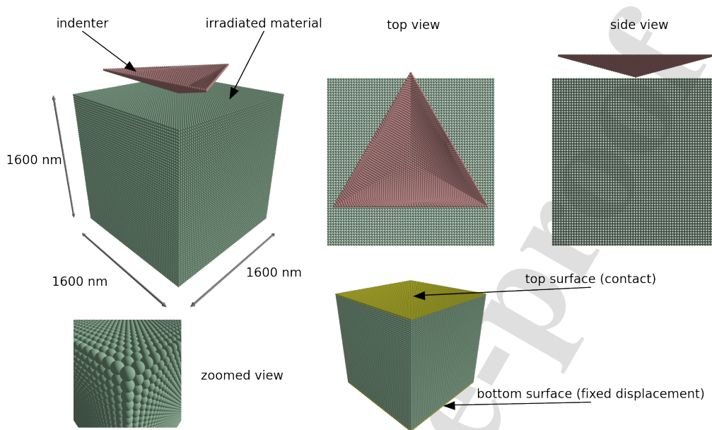
Figure 13: Discretized peridynamics model of indentation test
