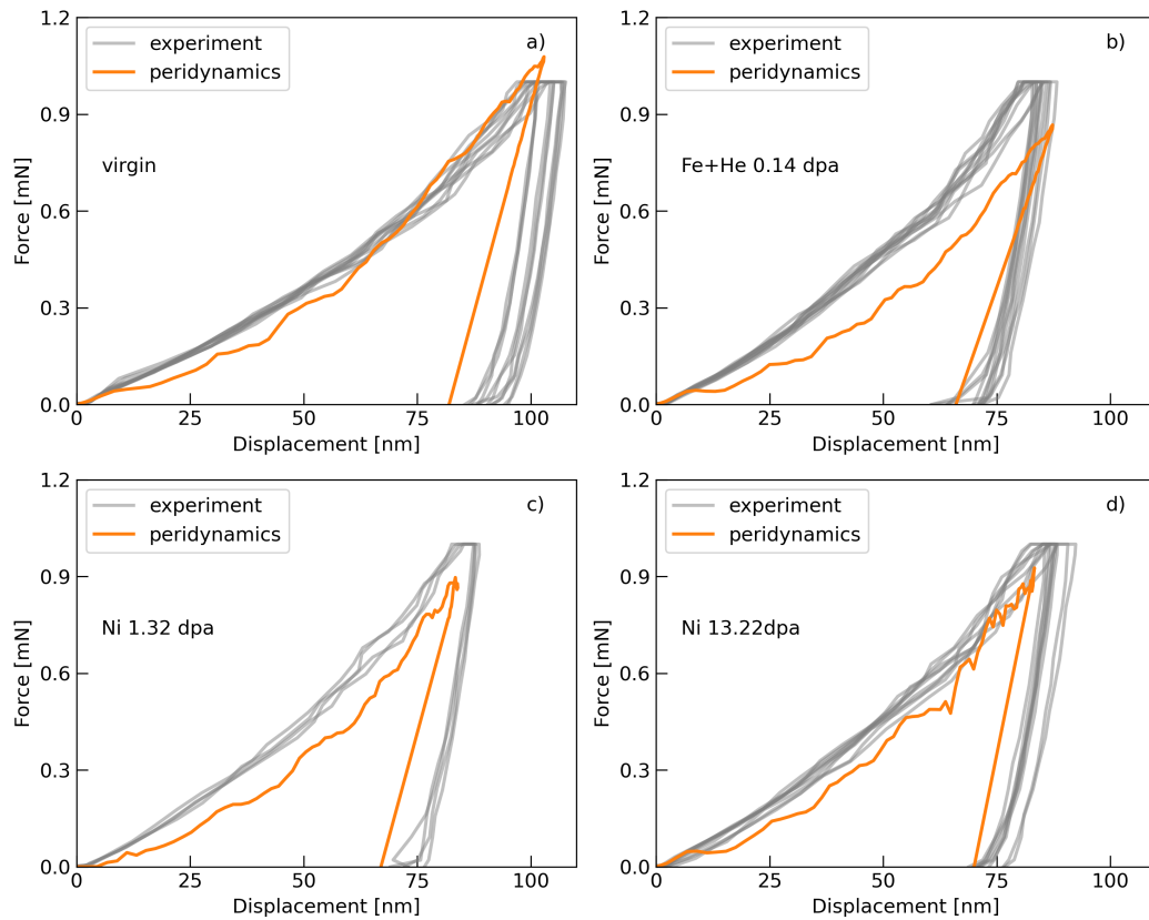
Figure 16: Comparison of the load – indentation depth curves between the experimental results and the numerical simulations for a) virgin material and b-d) different values of dpa
