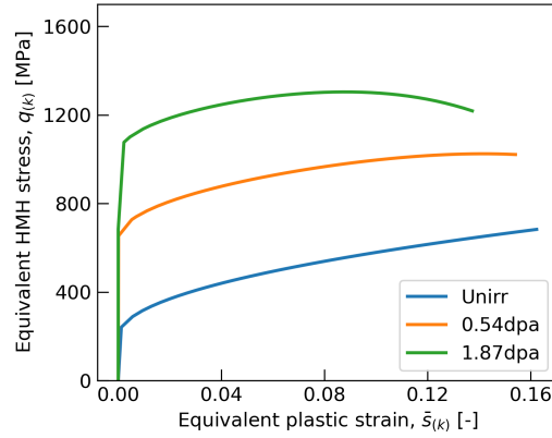
Figure 12: Prediction of the proposed constitutive model for the uniaxial tension test with different initial level of irradiation
