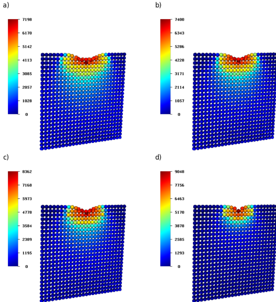
Figure 17: Distribution of equivalent HMM stress q_{(k)} at maximum indentation depth for several levels of dpa for a) unir b) irr1, c) irr2 and d) irr3. The units of stress is MPa
