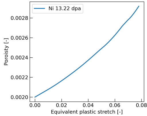
Figure 19: Evolution of radiation induced porosity as a function of equivalent plastic stretch
