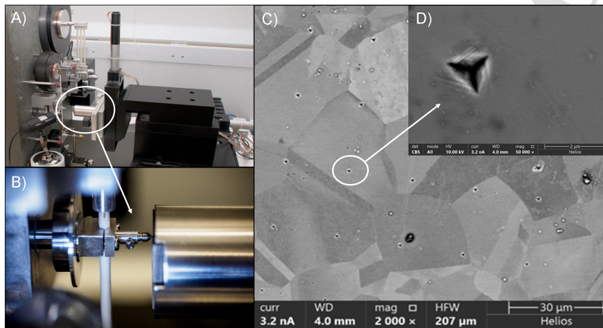
Figure 7: A) indenter system provided by MicroMaterials Ltd. B) snapshot of the indentation test C) SEM image of the 310S sample surface after indentation with 5 mN load and D) SEM image of the indent with visible characteristic slip planes developed during material deformation while loading
