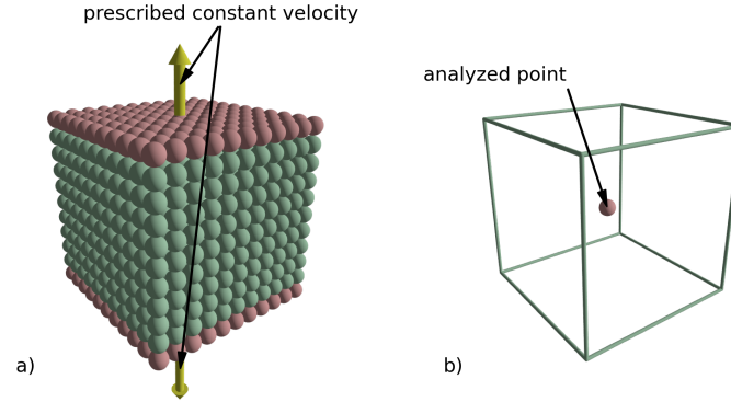
Figure 10: a) Schematic of the initial configuration of the peridynamics particles with marked boundary conditions for the peridynamic simulations of tensile tests b) location of the analyzed peridynamics particle
