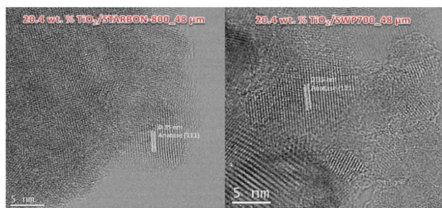
Figure 5. HR-TEM micrographs of 20.4 wt.% TiO 2 /STARBON-800_48 μm and 20.4 wt.% TiO 2 /SWP700_48 μm.
