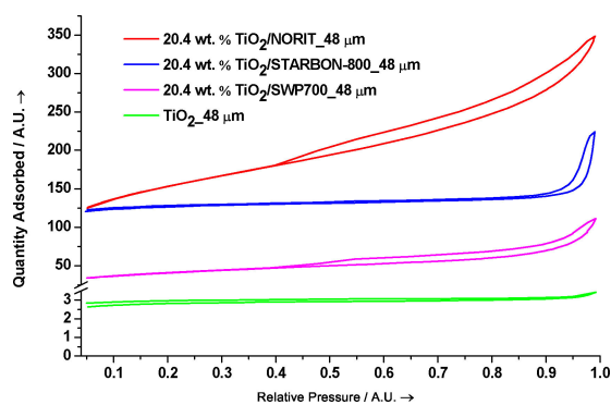
Figure 1. Nitrogen adsorption-desorption isotherms over all prepared materials.
