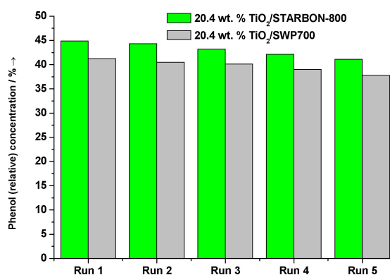
Figure 7. Multi-cycle performance of 20.4 wt.% TiO 2 /STARBON-800_48 μm and 20.4 wt.% TiO 2 /SWP700_48 μm photocatalysts in degradation of phenol in aqueous.
