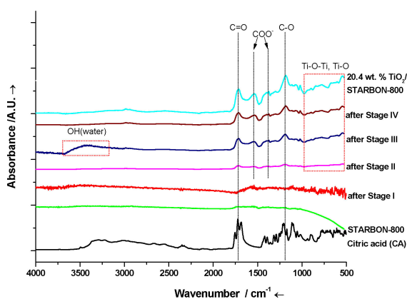
Figure 11. FTIR spectra of pure Citric acid (CA), STARBON-800, and materials from individual stages of 20.4 wt.% \text{TiO}_2 /STARBON-800 synthesis (ultrasound amplitude = 48 \mu\text{m} ).
