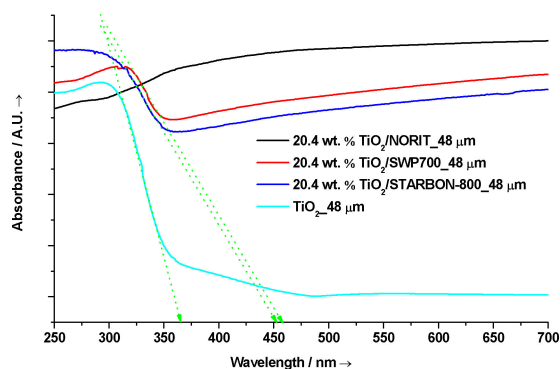
Figure 3. Diffuse reflectance UV-visible spectra of all prepared photocatalysts: 20.4 wt.% TiO 2 /SWP700_48 μm ("red line"), 20.4 wt.% TiO 2 /NORIT_48 μm ("black line"), 20.4 wt.% TiO 2 /STARBON-800_48 μm ("blue line") and TiO 2 _48 μm ("turquoise line").
