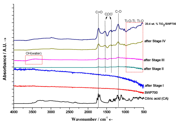
Figure 10. FTIR spectra of pure Citric acid (CA), SWP700, and materials from individual stages of 20.4 wt.% \text{TiO}_2 /SWP700 synthesis (ultrasound amplitude = 48 \mu\text{m} ).
