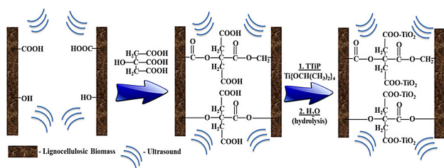
Figure 12. A diagram of the plausible formation of crystalline \text{TiO}_2 on lignocellulosic carbon materials prepared via ultrasound-assisted sol-gel method.
