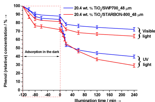
Figure 6. Photocatalytic phenol degradation under UV and visible light for TiO 2 /STARBON-800_48 μm and TiO 2 /SWP700_48 μm after optimization (error bars showing mean deviation of three experimental results).
