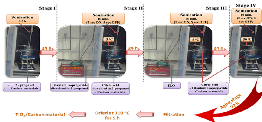
Figure 13. Synthesis procedure for composite \text{TiO}_2 /carbon materials using ultrasound-assisted sol-gel method [37] .
