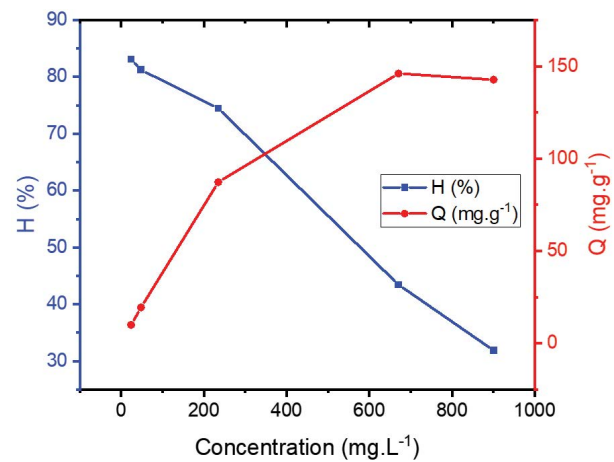
Fig. 13. Effect of initial Congo red concentration ( m = 0.10 \text{ g} , \text{pH}_0 = 6.55 , t = 4 \text{ h} ).
