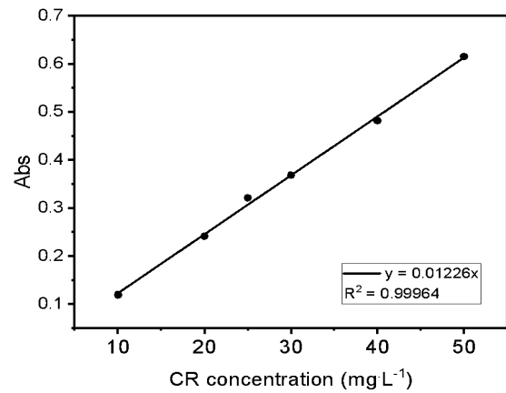
Fig. 7. Calibration curves of Congo red.
