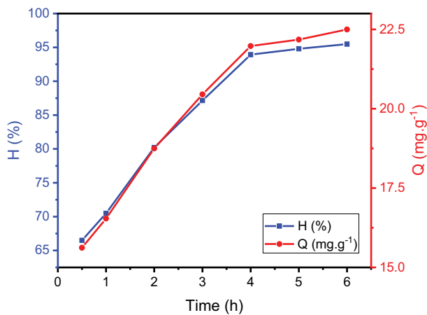
Fig. 9. Effect of contact time ( C_0 = 50 \text{ mg}\cdot\text{L}^{-1} , \text{pH}_0 = 6.55 , m = 0.10 \text{ g} ).
