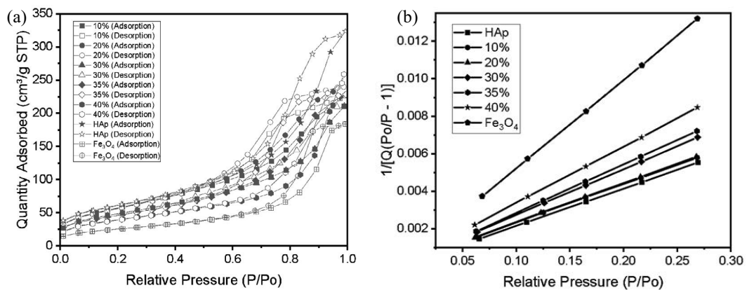
Fig. 5. \text{N}_2 adsorption-desorption isotherms (a) and Brunauer-Emmett-Teller plots (b) of HAp, \text{Fe}_3\text{O}_4 , and \text{Fe}_3\text{O}_4/\text{HAp} with different ratios.
