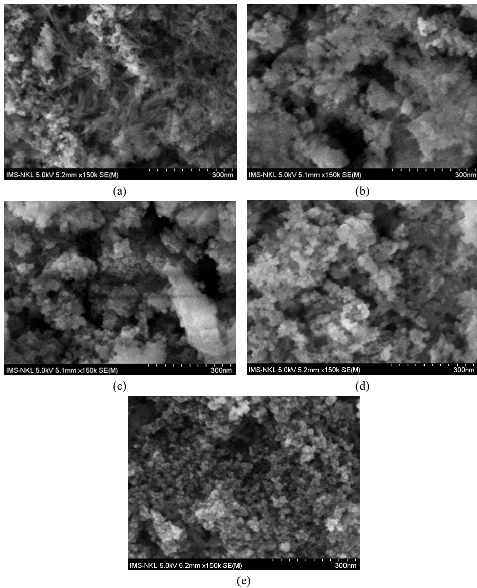
Fig. 4. Scanning electron microscopy images of 10%- \text{Fe}_3\text{O}_4/\text{HAp} (a), 20%- \text{Fe}_3\text{O}_4/\text{HAp} (b), 30%- \text{Fe}_3\text{O}_4/\text{HAp} (c), 35%- \text{Fe}_3\text{O}_4/\text{HAp} (d), and 40%- \text{Fe}_3\text{O}_4/\text{HAp} (e).
