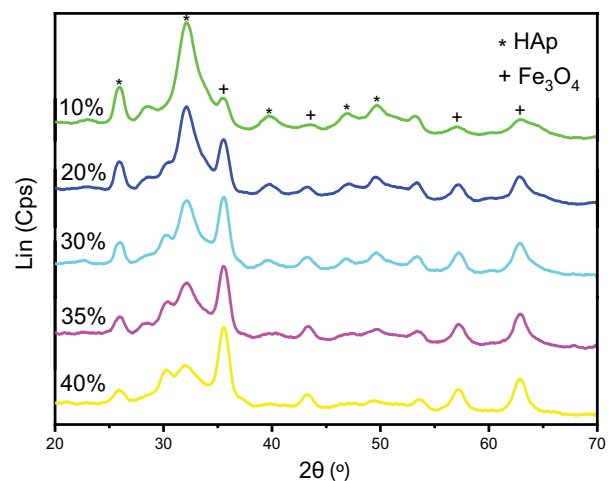
Fig. 2. X-ray diffraction patterns of \text{Fe}_3\text{O}_4/\text{HAp} .
