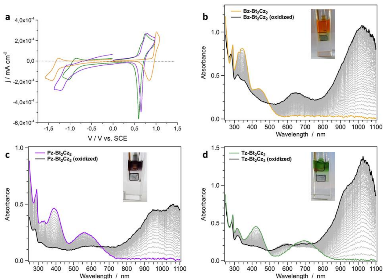
Figure 3. (a) Cyclic voltammograms at a scan rate of 100 \text{ mV s}^{-1} and (b-d) spectroelectrochemical experiments at a constant voltage of ( E^{\circ}_{\text{ox}} + 0.1 ) V vs. SCE. Both measurements were carried out in dichloromethane solution at 298 K; color code: Bz-Bt 2 Cz 2 (orange), Pz-Bt 2 Cz 2 (violet), and Tz-Bt 2 Cz 2 (green).
