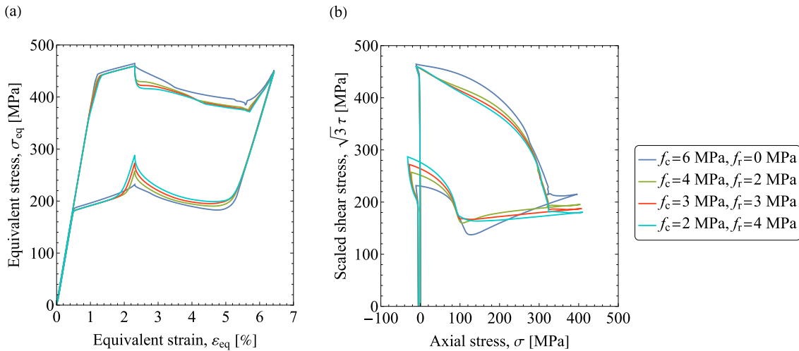
Fig. 6. NiTi tube under torsion (4%) followed by tension (6%): the effect of the dissipation parameters f_c and f_r on (a) the equivalent stress–equivalent strain response and (b) shear stress–axial stress response.
