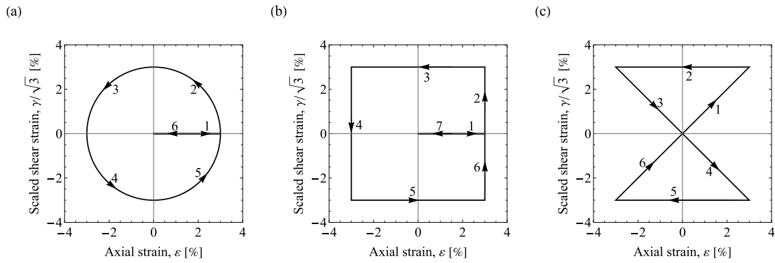
Fig. 1. Axial-shear strain paths used in the material-point analysis: (a) circular-shaped, (b) box-shaped, and (c) butterfly-shaped. The maximum axial strain and the maximum (scaled) shear strain in all cases is limited to 3% while the corresponding mean strains are zero.
