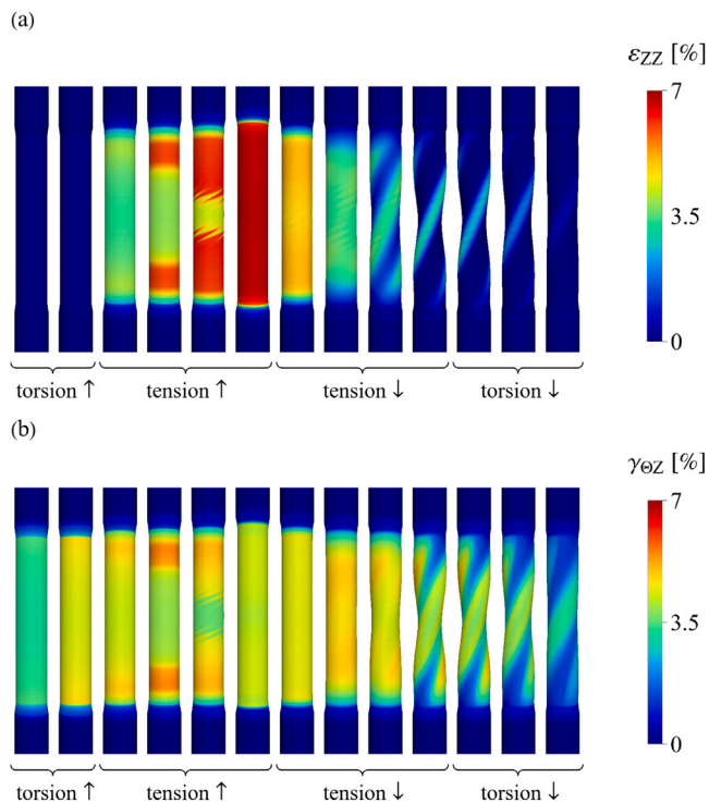
Fig. A.1. NiTi tube under torsion (4%) followed by tension (6%) exhibiting helical buckling: snapshots of the axial strain field \varepsilon_{zz} (a) and shear strain field \gamma_{\theta z} (b) for the simulation with the dissipation parameters f_c = 3 MPa and f_r = 3 MPa.
