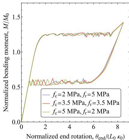
Fig. 12. NiTi tube under bending: bending moment–end rotation response obtained for different combinations of dissipation parameters f_c and f_r .
