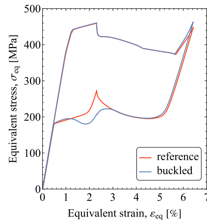
Fig. A.2. NiTi tube under torsion (4%) followed by tension (6%): comparison of the mechanical responses for the reference case and the case that exhibits buckling. The reference case is the one for the thicker tube analyzed in Section 4.2.
