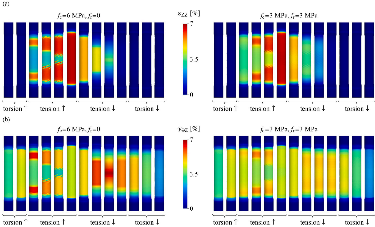
Fig. 7. NiTi tube under torsion (4%) followed by tension (6%): snapshots of the axial strain field \varepsilon_{zz} (a) and shear strain field \gamma_{\theta z} (b) for the simulations without and with the dissipation due to martensite reorientation, respectively, with f_c = 6 MPa and f_t = 0 (snapshots on the left) and f_c = 3 MPa and f_t = 3 MPa (snapshots on the right).
