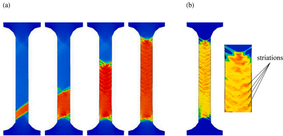
Fig. 14. Phase transformation evolution recorded in the experiment of Shariat et al. (2022): (a) representative snapshots of the transformation pattern during loading and (b) details of the transformation pattern at the end of loading, displaying clearly the striations. In both panels, the transformation is represented by the axial strain field, however, the color scale used in panel (b) is manipulated to enhance the visibility of striations. The figure is reproduced with permission from Elsevier.
