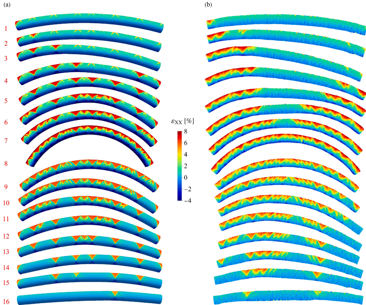
Fig. 9. NiTi tube under bending: comparison between (a) the predicted transformation evolution and (b) the transformation evolution observed in the experiment of Bechle and Kyriakides (2014) . The experimental snapshots are taken from the paper of Jiang et al. (2017a) (reproduced with permission from Elsevier). The numbers marking the simulation snapshots correspond to those indicated on the mechanical response in Fig. 8(a) .
