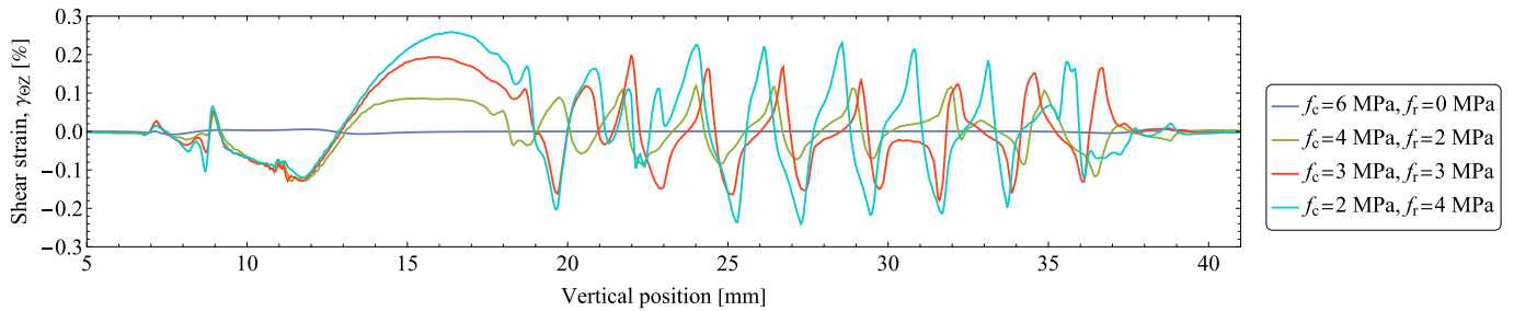
Fig. 17. Distribution of the shear strain \gamma_{\theta z} along the centerline of the dog-bone at the end of the loading stage. The plot corresponds to the gauge segment of the dog-bone.
