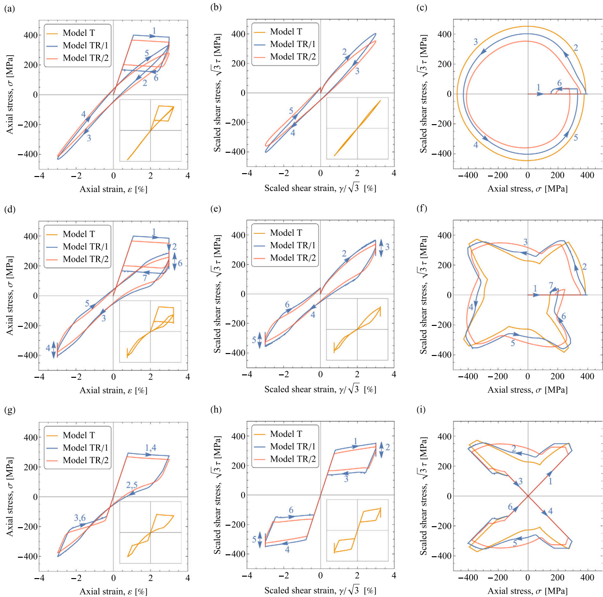
Fig. 2. Material-point responses obtained for different dissipation potentials under different axial-shear strain paths: (a,b,c) circular-shaped path, (d,e,f) box-shaped path, and (g,h,i) butterfly-shaped path. Panels (a,d,g) depict the axial stress-axial strain responses, panels (b,e,h) depict the shear stress-shear strain responses, and panels (c,f,i) depict the shear stress-axial stress responses. The superimposed arrows on the plots are solely intended to indicate the trajectories.
