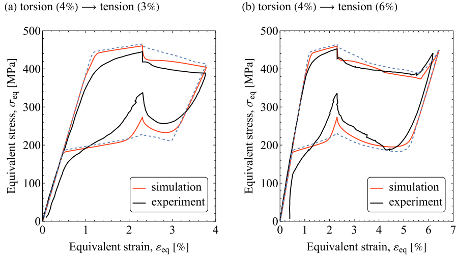
Fig. 4. NiTi tube under torsion-then-tension: the predicted equivalent stress–equivalent strain response compared with that from the experiment of McNaney et al. (2003). The blue dashed lines represent the simulation results with no dissipation due to reorientation, i.e., f_c = 6 MPa and f_t = 0 .
