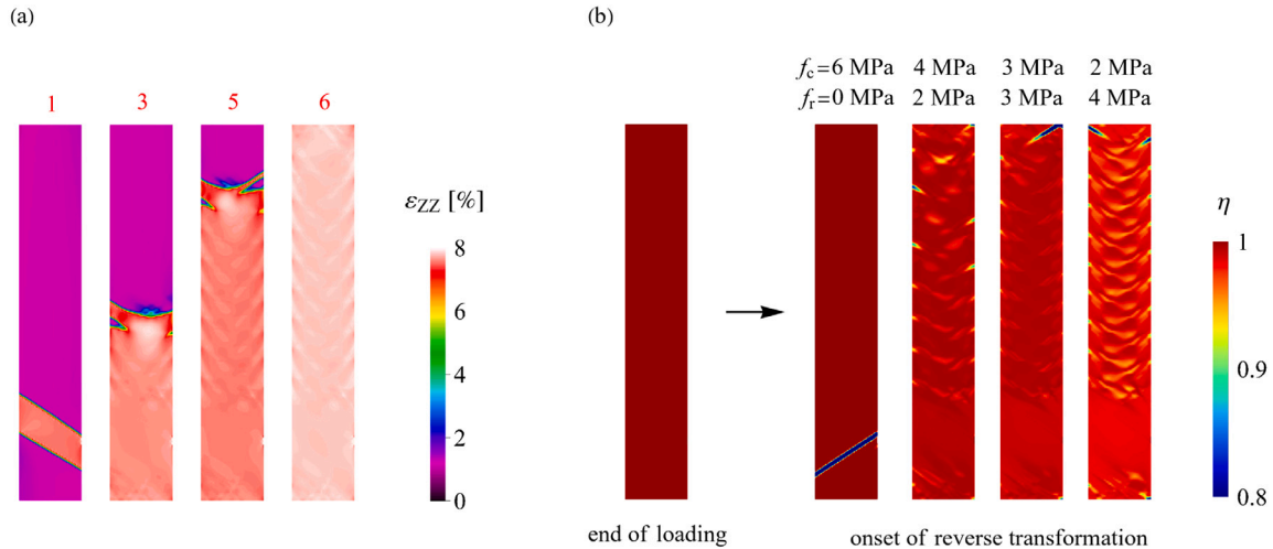
Fig. 18. NiTi strip under uniaxial tension: (a) the transformation pattern during loading for the reference dissipation parameters f_c = 3 MPa and f_r = 3 MPa, and (b) the effect of the dissipation parameters f_c and f_r on the pattern of the martensite volume fraction at the onset of the reverse transformation during unloading. The numbers in panel (a) refer to the same overall elongations as those indicated in Fig. 15(a).
