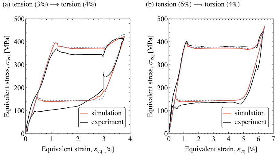
Fig. 5. NiTi tube under tension-then-torsion: the predicted equivalent stress–equivalent strain response compared with that from the experiment of McNaney et al. (2003). The blue dashed lines represent the simulation results with no dissipation due to reorientation, i.e., f_c = 6 MPa and f_t = 0 .
