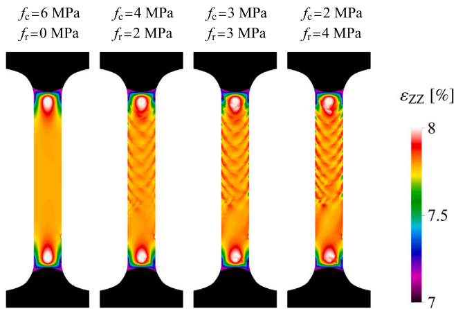
Fig. 16. NiTi dog-bone under uniaxial tension: a more detailed look at the transformed domain at the end of loading for different combinations of the dissipation parameters f_c and f_r .
