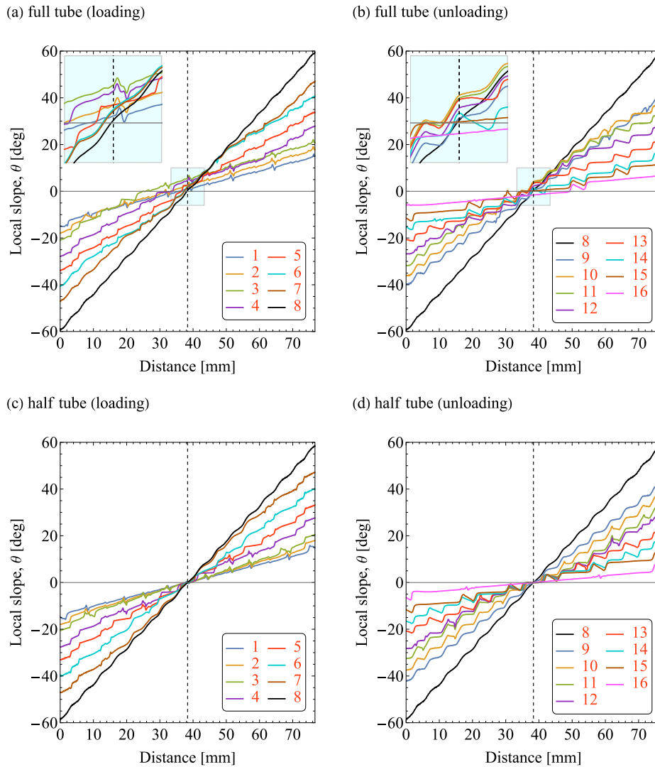
Fig. 11. NiTi tube under bending: distribution of the slope along the tube at various stages of loading and unloading for (a,b) full tube and (c,d) half tube. The numbers in the legends correspond to the deformation stages shown in Fig. 10. For the ease of comparison, the plots related to half tube are reflected along the plane of symmetry (mid-span) and are shown as full. The vertical dashed line indicates the mid-span of the undeformed tube.
