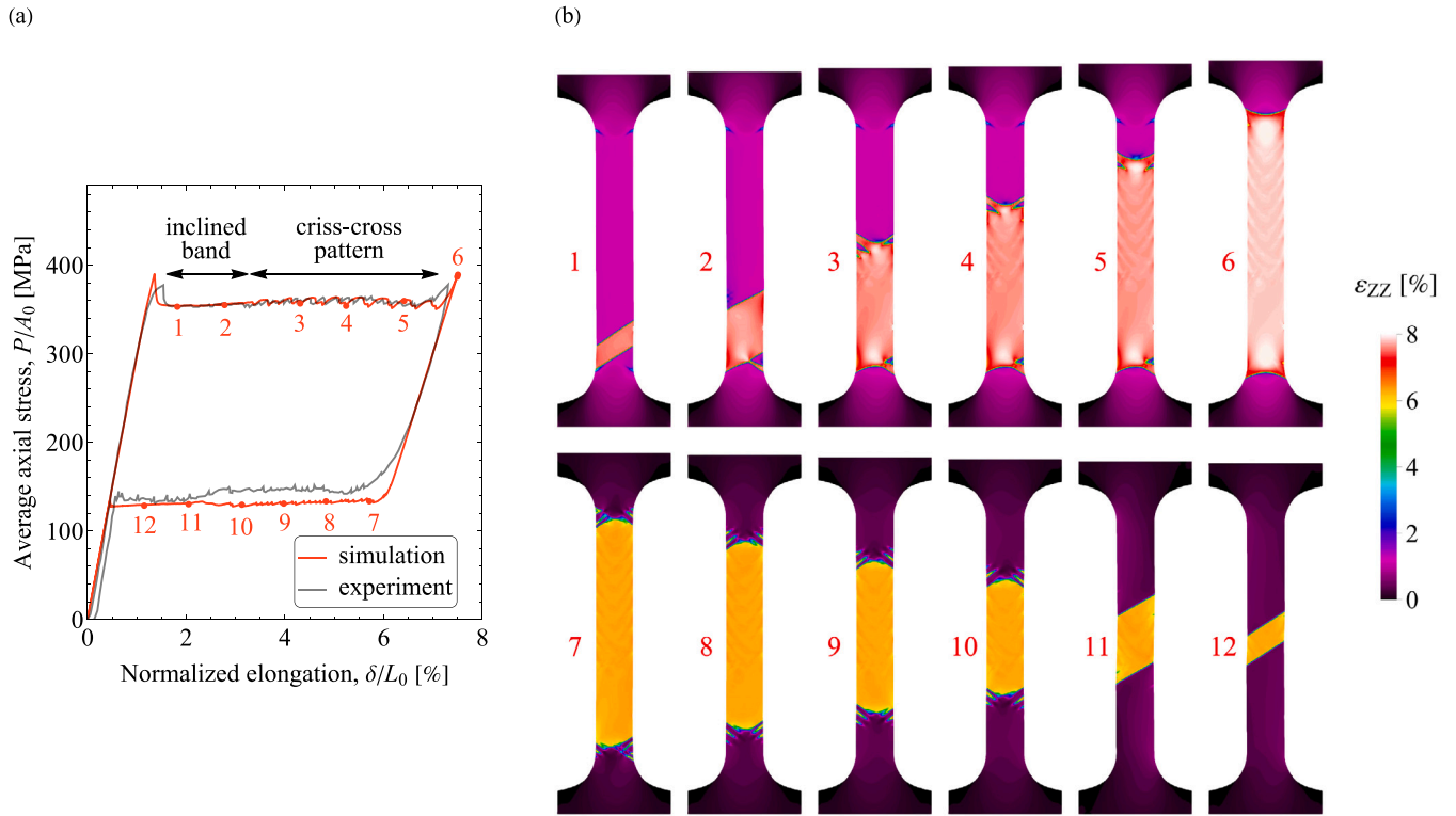
Fig. 15. NiTi dog-bone under uniaxial tension: (a) mechanical response and (b) transformation pattern. The experimental response in panel (a) refers to Shariat et al. (2022), and the corresponding transformation pattern is depicted in Fig. 14.
