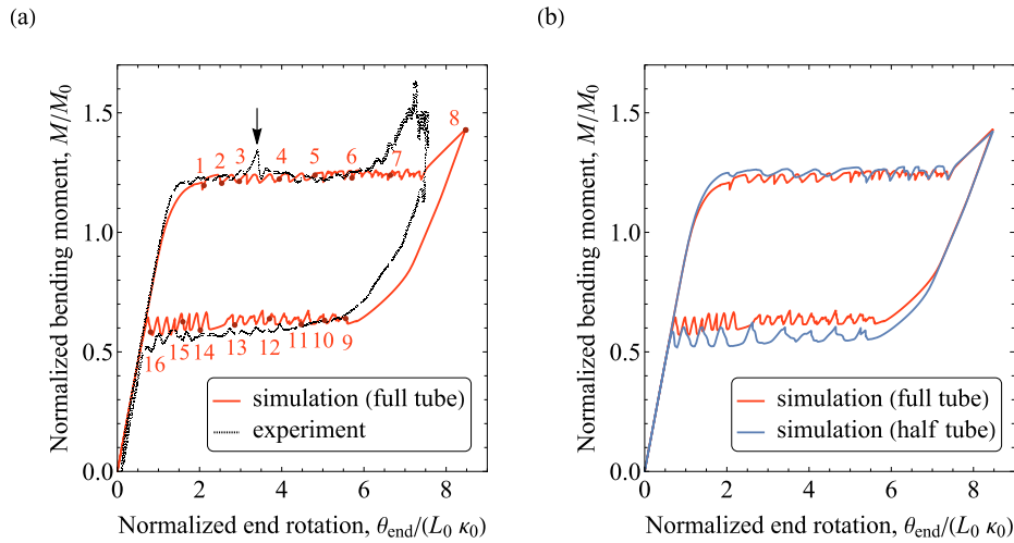
Fig. 8. NiTi tube under bending: (a) comparison between the predicted bending moment–end rotation response with that from the experiment of Bechle and Kyriakides (2014) and (b) comparison between the bending moment–end rotation responses obtained for the simulations with full tube and half tube.
