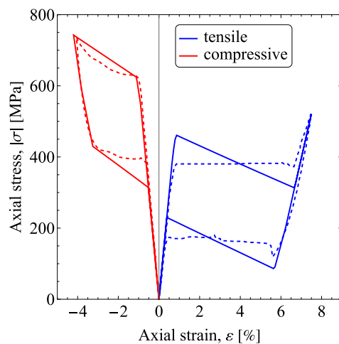
Fig. 3. The intrinsic response in tension and compression calibrated for the numerical example of NiTi tube under pure bending (Section 4.3). The dashed curves represent the structural responses obtained in the experiment of Bechle and Kyriakides (2014) at 23°.
