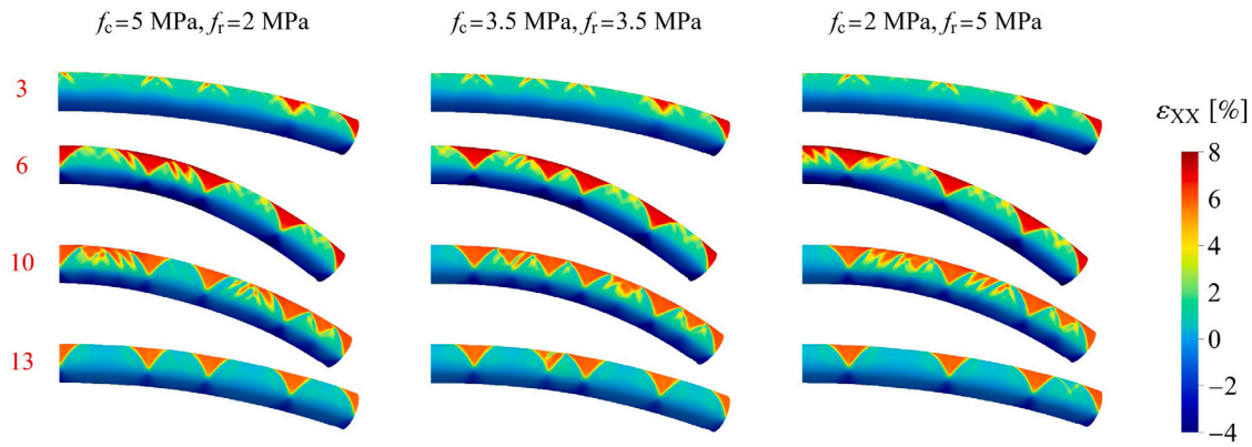
Fig. 13. NiTi tube under bending: predicted transformation pattern for different combinations of dissipation parameters f_c and f_r . The numbers marking the snapshots correspond to the same end rotations as those indicated on the mechanical response in Fig. 8.
