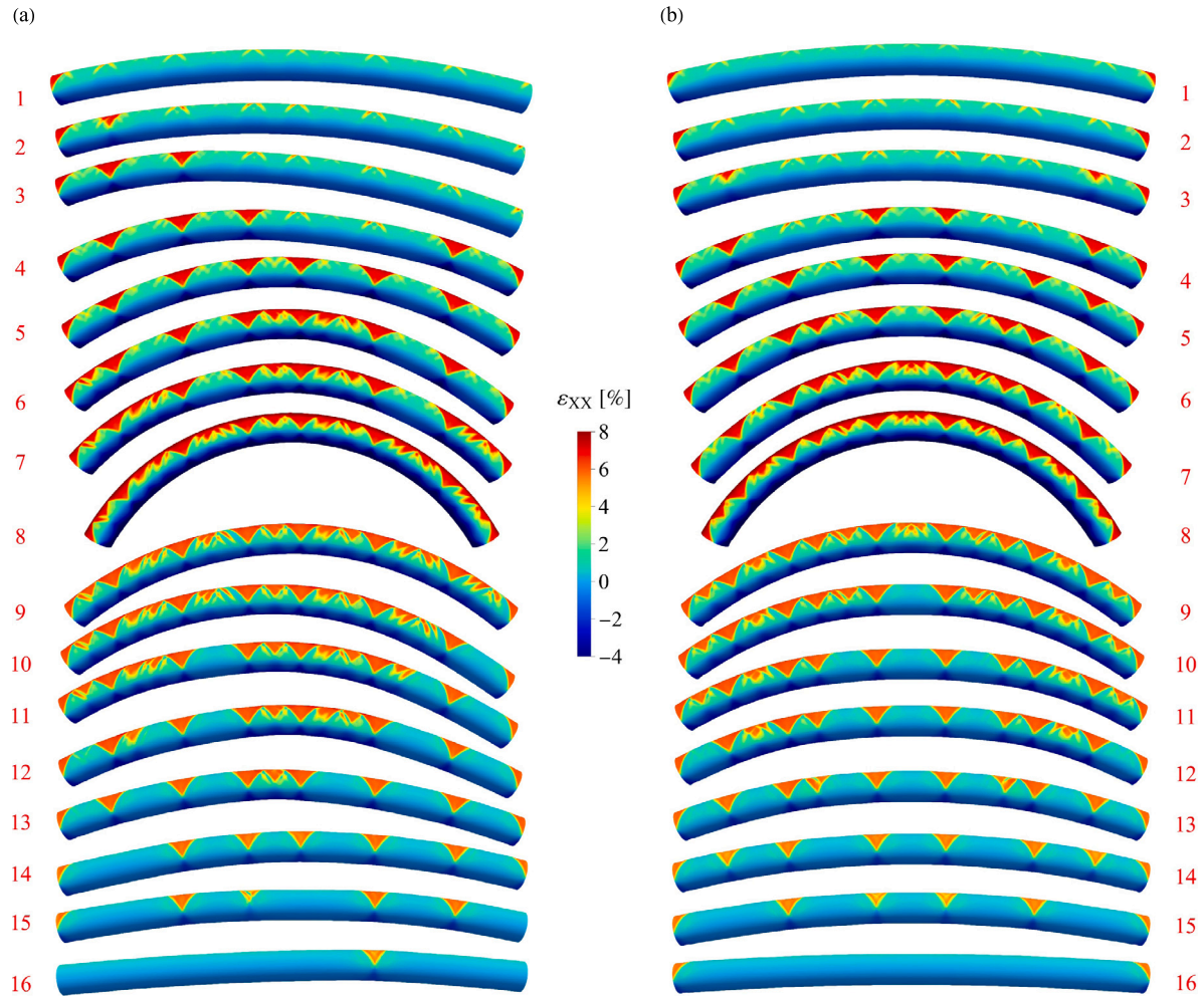
Fig. 10. NiTi tube under bending: comparison between the transformation evolutions in the simulations with (a) full tube and (b) half tube. For the ease of comparison, the half tube is reflected along the plane of symmetry (mid-span) and is shown as full. The snapshots correspond to nearly the same prescribed angle \theta_{\text{end}} .
