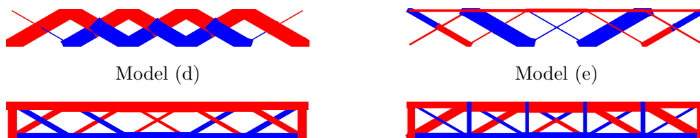
Model (f) (Scale up to 5 times for thickness) Model (g) (Scale up to 5 times for thickness)
