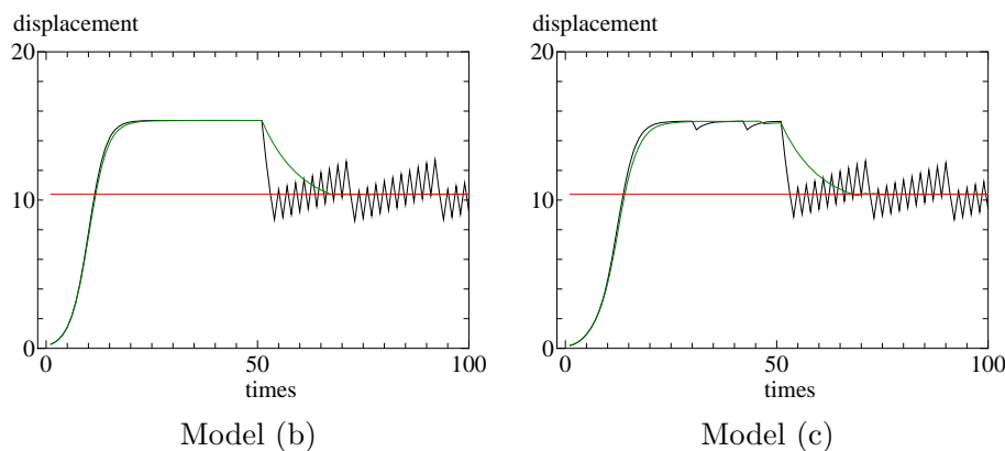
Figure 4. A scissors unit central displacement
