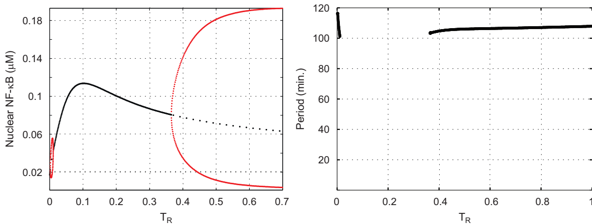
Fig. 4. The bifurcation diagram for T_R when \text{totalNF}\kappa\text{B} = 0.15 \mu\text{M} : there are three HB-points at T_R = 0.002, 0.01 and 0.366 , respectively. Sustained oscillations occur for values of T_R in either of the intervals (0.002, 0.01) and (0.366, 1] . The right panel shows the period of these oscillations.
