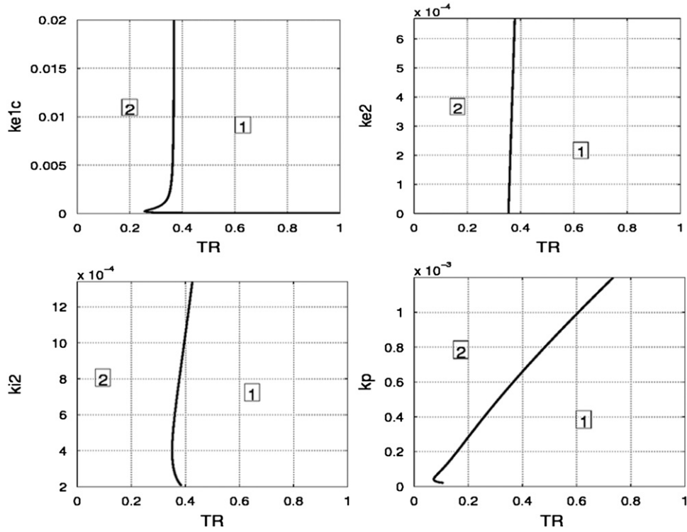
Fig. C4. The two-parameter bifurcation diagrams for T_R and k_{e1c} , k_{e2} , k_{i2} and k_p , in which the curves trace out the locations of Hopf bifurcation points. These curves divide the parameter space into two types of regions: limit cycle region is marked by 1 and steady-state region marked by 2.
