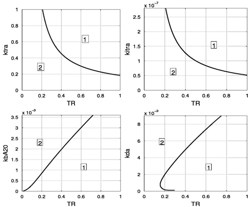
Fig. C5. The two-parameter bifurcation diagrams for T_R and k_{tra} , ki_{tra} , kbA20 and k_{da} , in which the curves trace out the locations of Hopf bifurcation points. These curves divide the parameter space into two types of regions: limit cycle region is marked by 1 and steady-state region marked by 2.
