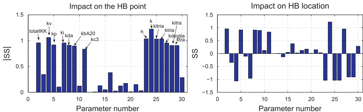
Fig. 5. Sensitivity scores for the 26 reaction rates and the two concentration parameters ( \tau_{totalNF\kappa B} and \tau_{totalIKK} ) constructed using Eq. (4) with \theta = 0.1 : (left) absolute value of the sensitivity score against parameter number (see Table 1) and (right) sensitivity score against the index of parameters.
