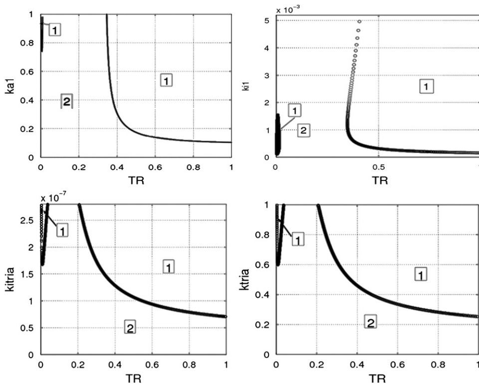
Fig. C2. The two-parameter bifurcation diagrams for T_R and k_{a1} , k_{i1} , k_{itria} and k_{tria} , in which the curves trace out the locations of Hopf bifurcation points. These curves divide the parameter space into two types of regions: limit cycle region is marked by 1 and steady-state region marked by 2.
