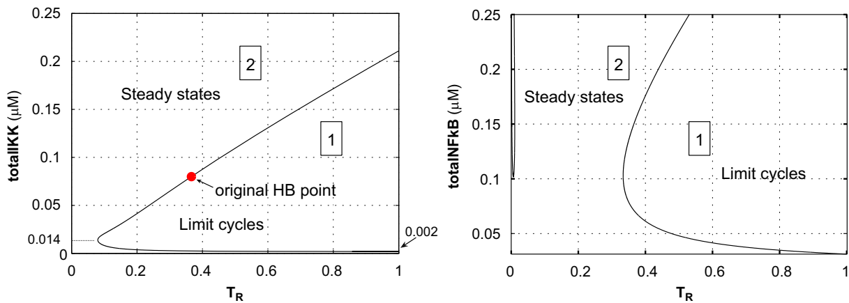
Fig. 3. The two-parameter bifurcation diagrams for T_R and \text{totalIKK} (left panel) and T_R and \text{totalNF}\kappa\text{B} (right panel). Here each point on the curves represents a HB-point and the curves divide the parameter spaces into two types of region: there is a limit cycle for each pair of the parameters in Region 1, in which and there is a non-oscillatory steady-state for each pair of parameters in Region 2.
