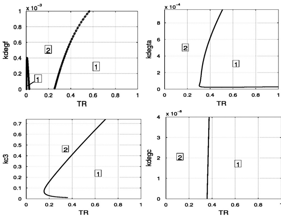
Fig. C3. The two-parameter bifurcation diagrams for T_R and k_{degf} , k_{degta} , kc_3 and k_{degc} , in which the curves trace out the locations of Hopf bifurcation points. These curves divide the parameter space into two types of regions: limit cycle region is marked by 1 and steady-state region marked by 2.
