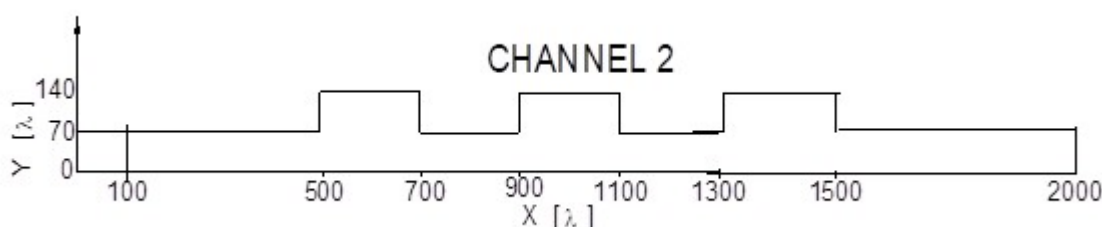
Figure 1. Optimum shape of the damper channel.
